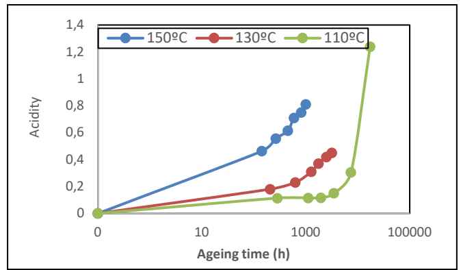
Figure 6. Acidity of mineral oil during ageing.
