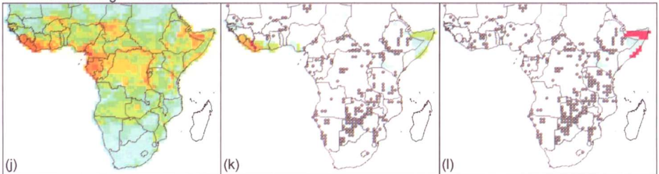
Fig. 2 Geographical patterns in Africa of all 946 species of mammal (top row), all 197 threatened mammal species (second row), all 194 large mammal species (third row), and all 51 threatened large mammal species (bottom row) at a one-degree resolution. The second and third columns illustrate gaps in protection of mammal species when at least 25% of a grid cell is protected by wildlife reserves and wildlife and forest reserves combined, respectively (grey dots show cells with <25% protection). See text for definition of wildlife and forest reserves.
