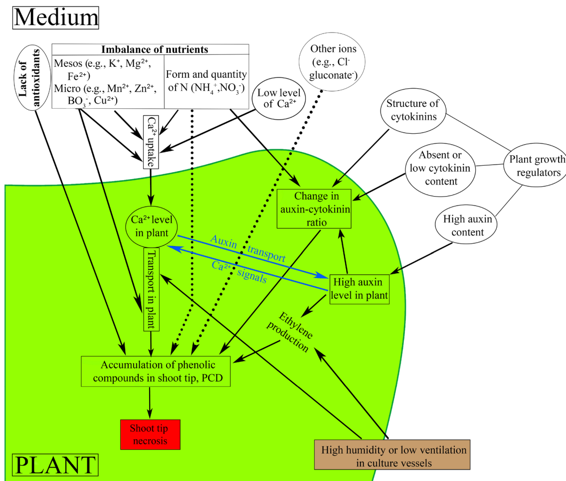
Fig. 6 Schematic diagram showing the overall mechanisms of shoot tip necrosis (STN) in in vitro plants. A detailed description may be found in the text, in "Conclusion"
