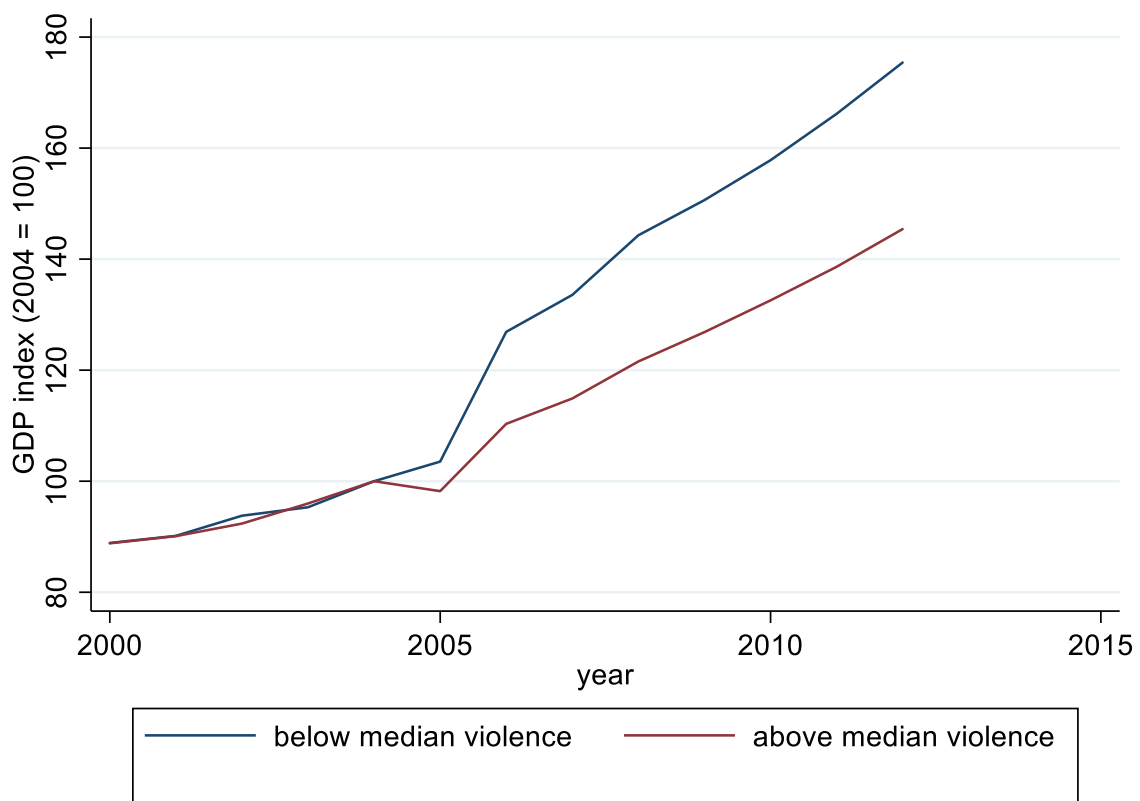
Figure 5: GDP dynamics in Aceh's districts experiencing above versus below median violence
