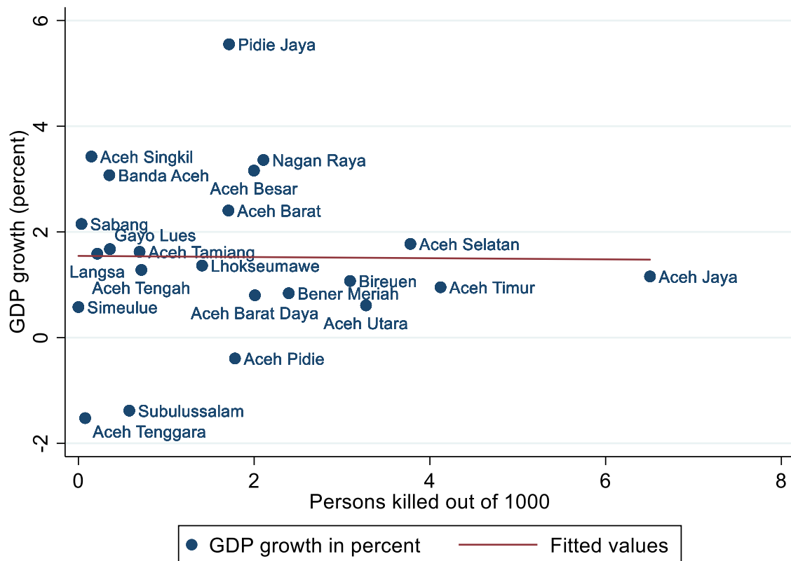
Figure 3: Wartime growth (2000-2004) versus wartime conflict casualties per capita (1999-2004) in Acehese districts
