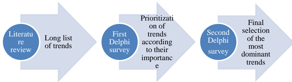
Figure 4.12: Steps in Phase 1 of the ANP
