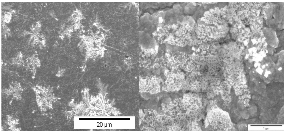
Figure 5.4 SEM image of the thin film of nanoporous gold on the surface of the sputtered gold.
