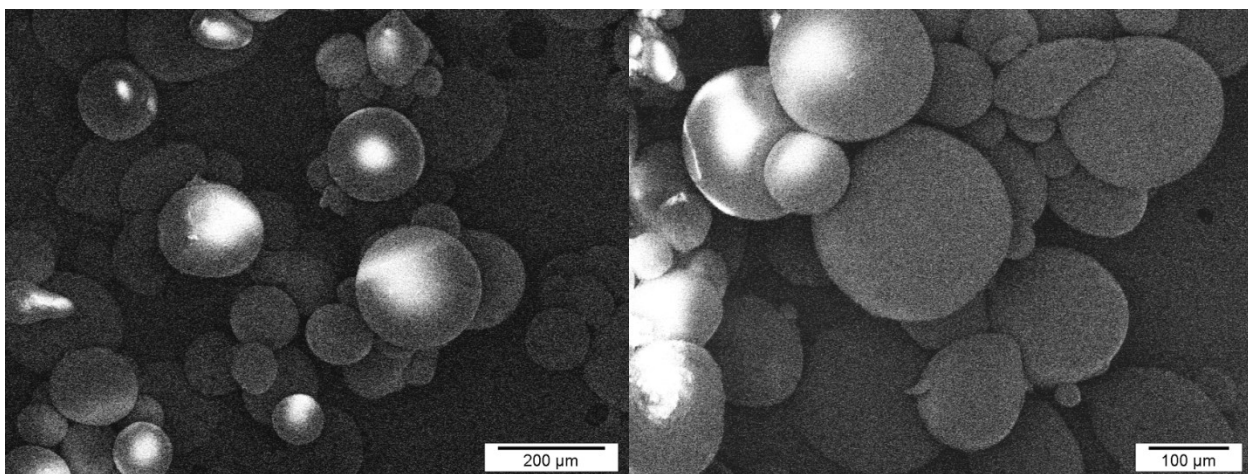
Figure 7.9. SEM image of polystyrene based polymer at: a) 100x and b) 150x magnifications
