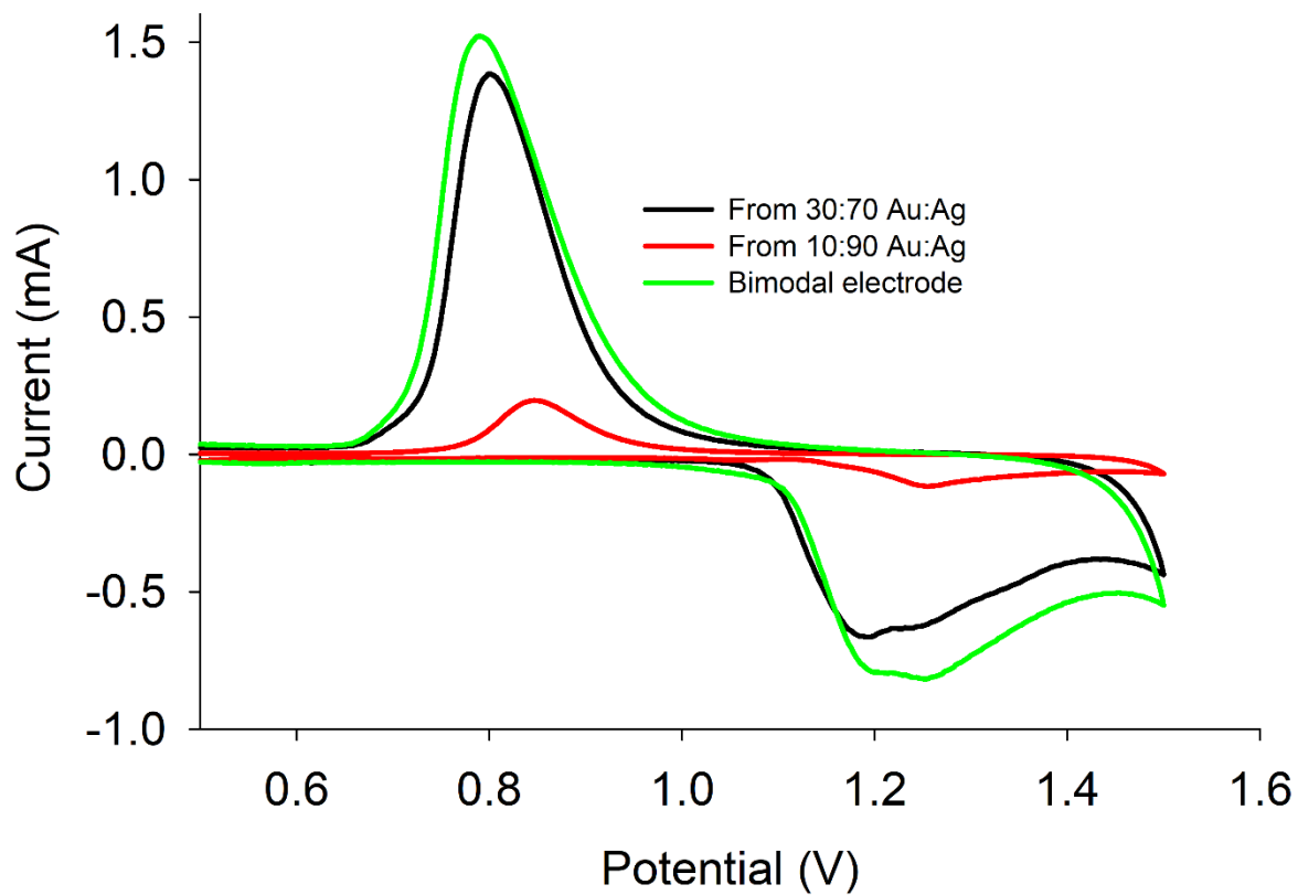
Figure 6.2 Cyclic voltammogram of NPG electrode NPG electrode from the dealloying of the gold alloy of the gold and silver at 30:70 ratio (black line), 10:90 ratio (red line) and
