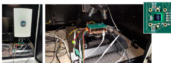
Fig. 7 ASIC laser radiation tests
