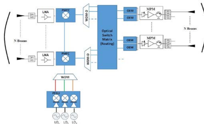
Fig. 1 Simplified payload block diagram using photonic equipment
