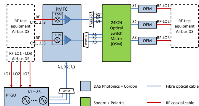
Fig. 2 OPTIMA demonstrator architecture
