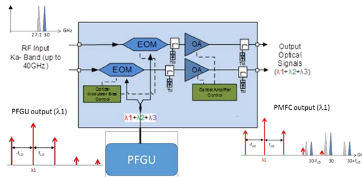
Fig. 4 Block diagram of photonic multi-frequency converter (PMFC)
