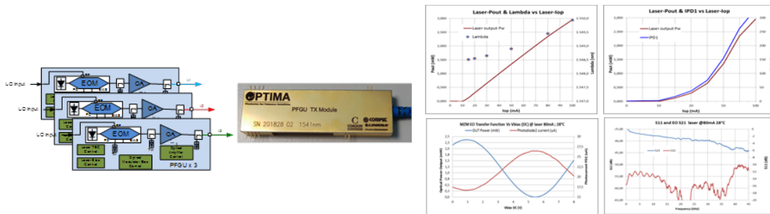
Fig. 3 Block diagram of photonic frequency generation unit (left), picture of the co-packaged laser modulator device (center) and simulated and measured characteristic curves of the PFGU Tx module (right).
