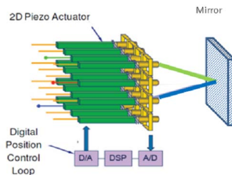
Fig. 6 DirectLight® core technology with mirror reflection based configuration
