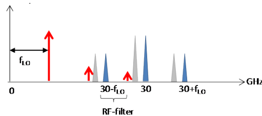
Fig. 5 IF spectrum after optoelectronic conversion
