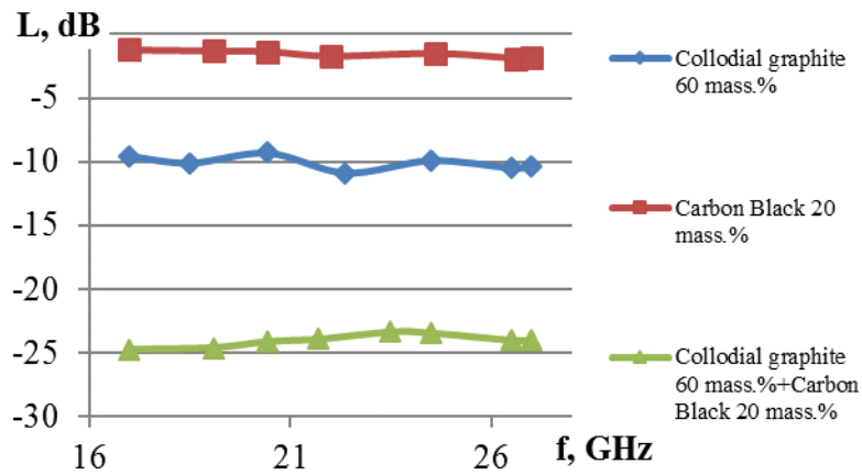
Fig. 1. Electromagnetic losses for carbon materials and their blends
