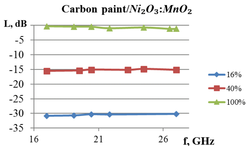
Fig. 2. Effects of the amount of oxide mixture on electromagnetic characteristics of composite
