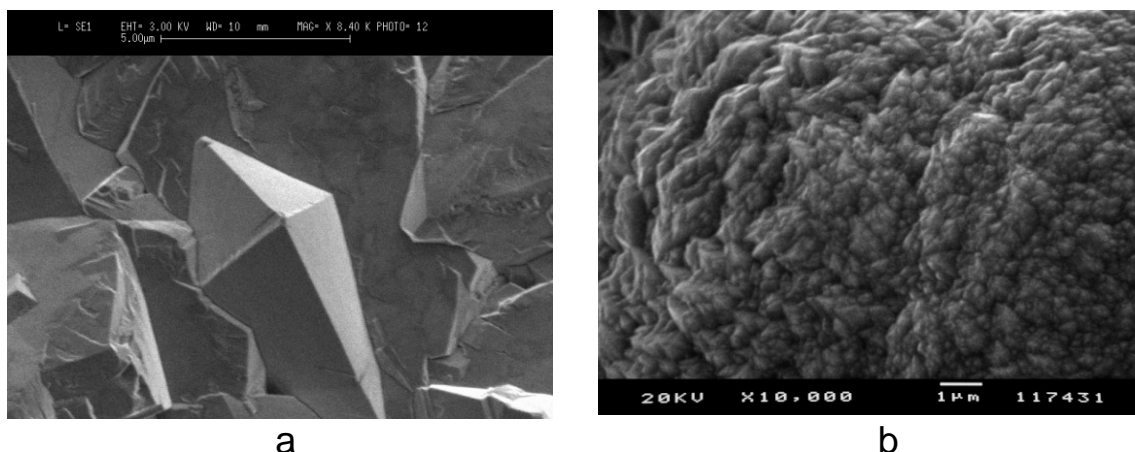
Fig. 1. SEM micrographs of coatings, obtained from next solutions: a – 0.1 M \text{Pb}(\text{NO}_3)_2 + 0.1 M \text{HNO}_3 ; b – 0.1 M \text{Pb}(\text{CH}_3\text{SO}_3)_2 + 0.1 M \text{CH}_3\text{SO}_3\text{H}
