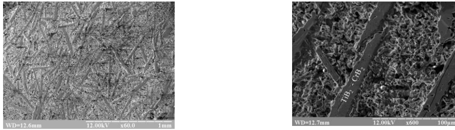
Fig. 1. The structure of primary cast alloy XTH40 with initial crystals of interstitial phase TiB_2-CrB_2
