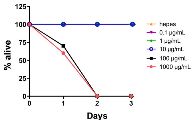
Fig. 1. Effects of purified Cry5B on H. contortus adults. Triple anthelmintic-resistant H. contortus adults were incubated in vitro with varying concentrations of purified Cry5B and scored for live or dead (no movement even after touch). Intoxication in this scoring scheme is seen at 100 and 1000 µg/mL. All other doses overlapped completely with HEPES control.
