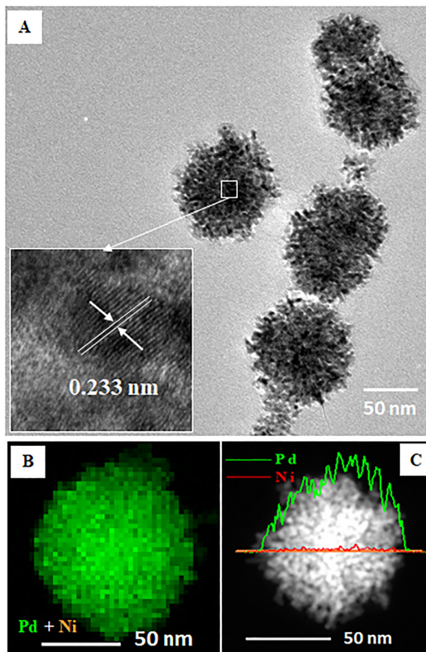
Fig. 4. (A) TEM images of Pd nanodendrites obtained from H_2PdCl_4/10 mM HCl after aging for 24 h. (B) Elemental EDX mapping of nanodendrite [orange denotes Ni and green denotes Pd]. (C) EDX line scan of nanodendrite. (For interpretation of the references to color in this figure legend, the reader is referred to the web version of this article.)
