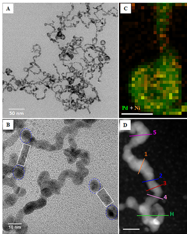
Fig. 3. TEM image and HR-TEM image of a tadpole with the calculated lattice fringes for the head and tail (node).
