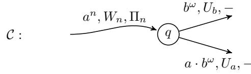
■ Figure 5 The state q and the notations from the proof of Theorem 5, for two different even n \in \mathbb{N} such that \delta(r_n[1..n]) = q . The labels on the walks indicate the input word and the accumulated weight and discount factors.
