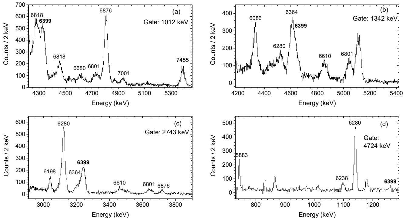
Figure 3: Transitions observed from the 6399-keV state. Gates at \gamma -ray energies of (a) 1012 keV, (b) 1342 keV, (c) 2743 keV, and (d) 4724 keV have been applied to observe transitions to 2^+ states at 2069 keV, 1759 keV, 3160 keV, and 5142 keV, respectively. The peaks have been labelled with excitation energies corresponding known excited states in ^{26}\text{Al} .
