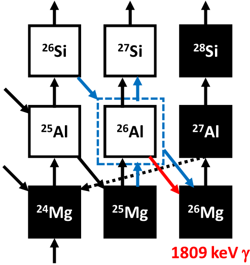
Figure 1: The Mg-Al hydrogen-burning reaction cycle. The arrows indicate the reaction flow via proton captures and \beta -decays. The 1809-keV \gamma ray follows the \beta -decay of the ^{26}\text{Al} ground state ( J^\pi = 5^+ , T_{1/2} = 0.7 My) highlighted in red. The bypass routes related to ^{26m}\text{Al} ( J^\pi = 0^+ , T_{1/2} = 6.35 s) are shown in blue. The black squares indicate stable isotopes and \beta -unstable nuclei are shown in white.
