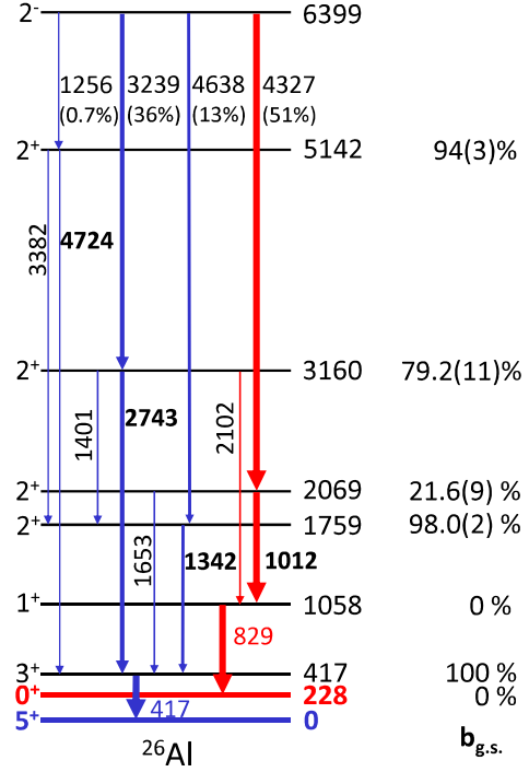
Figure 2: \gamma -ray transitions and their branchings observed from the 6399-keV state together with the gating transitions (in bold). The transitions going dominantly to the ground state and the isomer are shown in blue and red, respectively. The transitions observed in this work from the 6398.64(21)-keV [13] state have uncertainties of around 2 keV (see Table 1) and result in E_x = 6398.0(20) keV. Other intense \gamma -ray transitions ( I_\gamma \geq 10\% in [13]) are also indicated for the relevant states. The fraction of transitions populating the ground state either directly or via cascades from each level ( b_{g.s.} ) is based on the intensities from Ref. [13].
