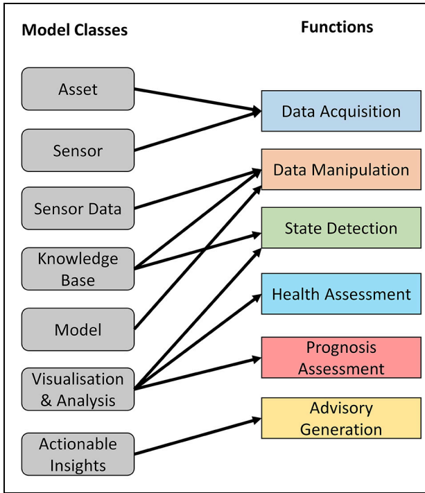
Figure 4. Ontology-functional mapping.
