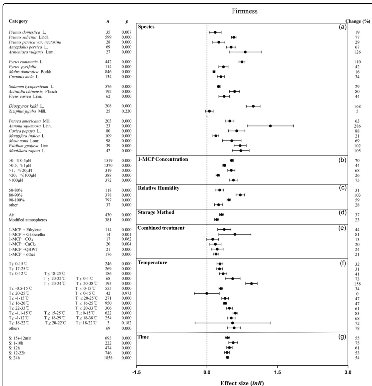
Fig. 4 Summary effects (as natural logs, \ln R ) and 95% confidence intervals (CIs) for the influence of 1-MCP treatment on firmness. Summary effects were analyzed in fruit exposed to 1-MCP, with the impacts of seven moderator variables on the magnitude of the treatment effect portrayed (a–g). Category list levels of each moderator. Change refers to the raw percentage increase in firmness induced by 1-MCP.
