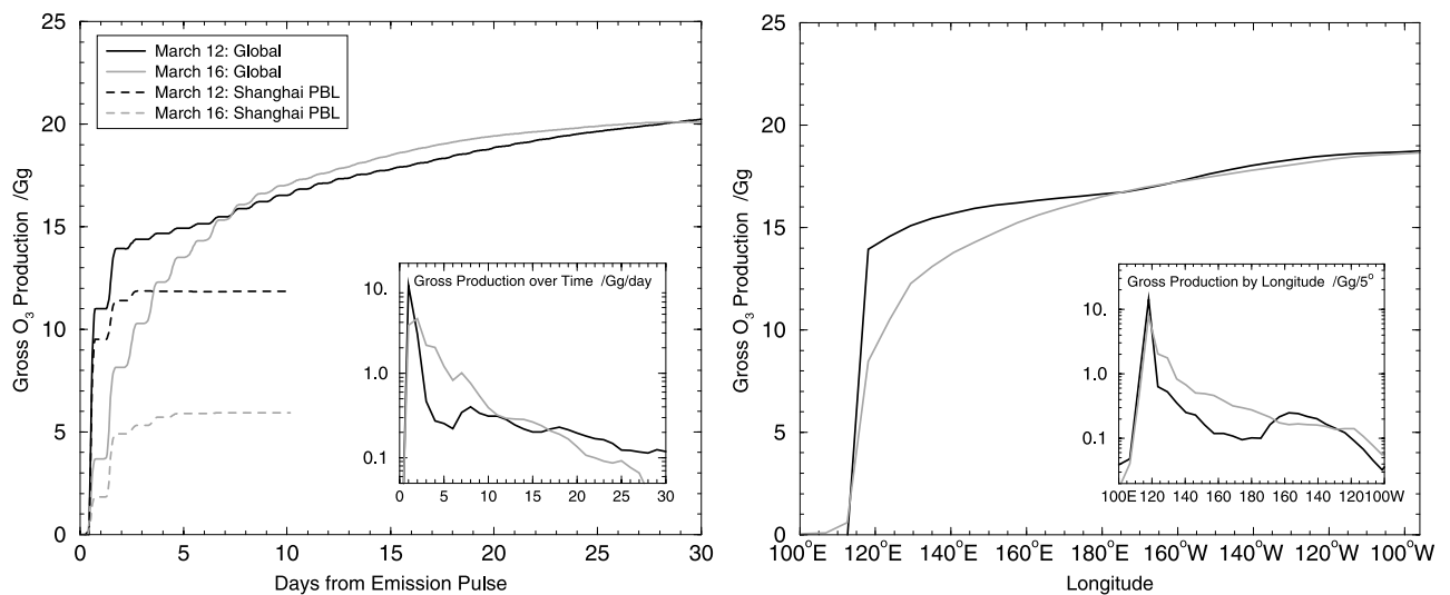
Figure 7. Cumulative additional O 3 formation (left) with time and (right) with longitude following 1 day's emissions of precursors from Shanghai on 12 March (black) and 16 March (grey), revealing the temporal and spatial evolution of gross production over the first month. Inserts show the absolute production on a log scale to highlight additional formation over the eastern Pacific after day 7 in the 12 March case
