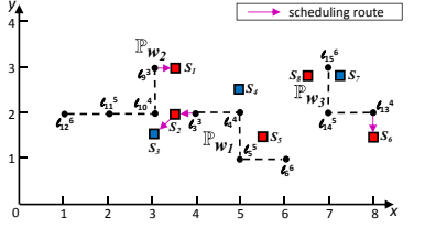
(a) Snapshot Routes by MTA
