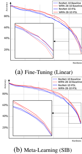
Figure 5: Accuracy across query hardness on 5-shot fine-tuning and meta-learning. Additional results are shown in Appendix 6.
