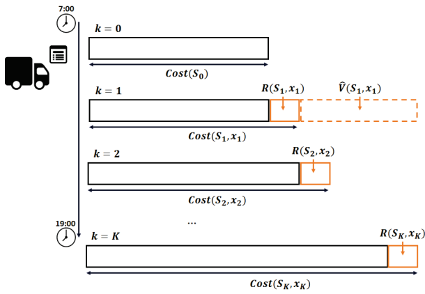
Figure 1: Illustration on how the reward function is derived.
