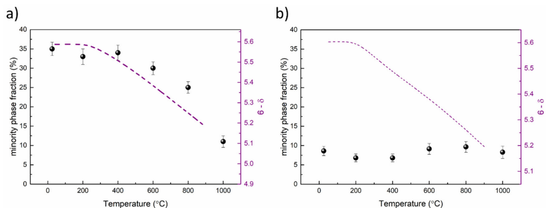
Figure 5. The fraction of the minority phases (dot) P4/m\bar{m}m for BLC (a) and Pm\bar{3}m for BNC (b), and oxygen stoichiometry (dashed line) as a function of temperature. The oxygen stoichiometry changes were calculated based on thermogravimetry using titration results as a starting point.
