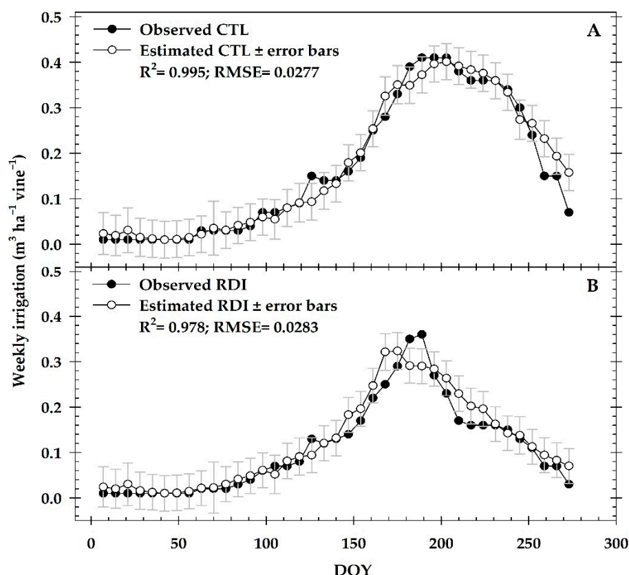
Figure 7. Estimated (white circles) and observed (black circles) weekly irrigation ( \text{m}^3 \cdot \text{ha}^{-1} \cdot \text{vine}^{-1} ) for CTL (A) and RDI (B) treatments referenced to the day of the year (DOY) for 2017.
