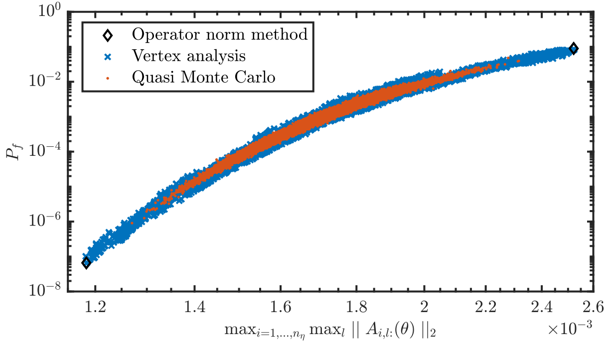
Figure 3: Results of the propagation of the uncertainty through the building model, obtained by performing a Vertex analysis (blue crosses), Quasi Monte Carlo sampling (orange dots) and the optimization approach (black diamonds).
