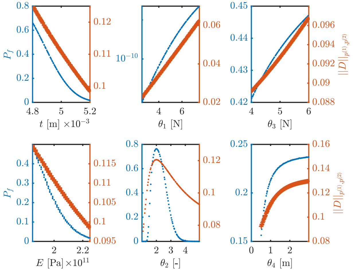
Figure 1: Effect of varying each parameter separately on the operator norm \|\mathbf{D}\|_{p^{(1)},p^{(2)}} (orange plus signs) as well as on the probability of failure P_f (blue dots)
