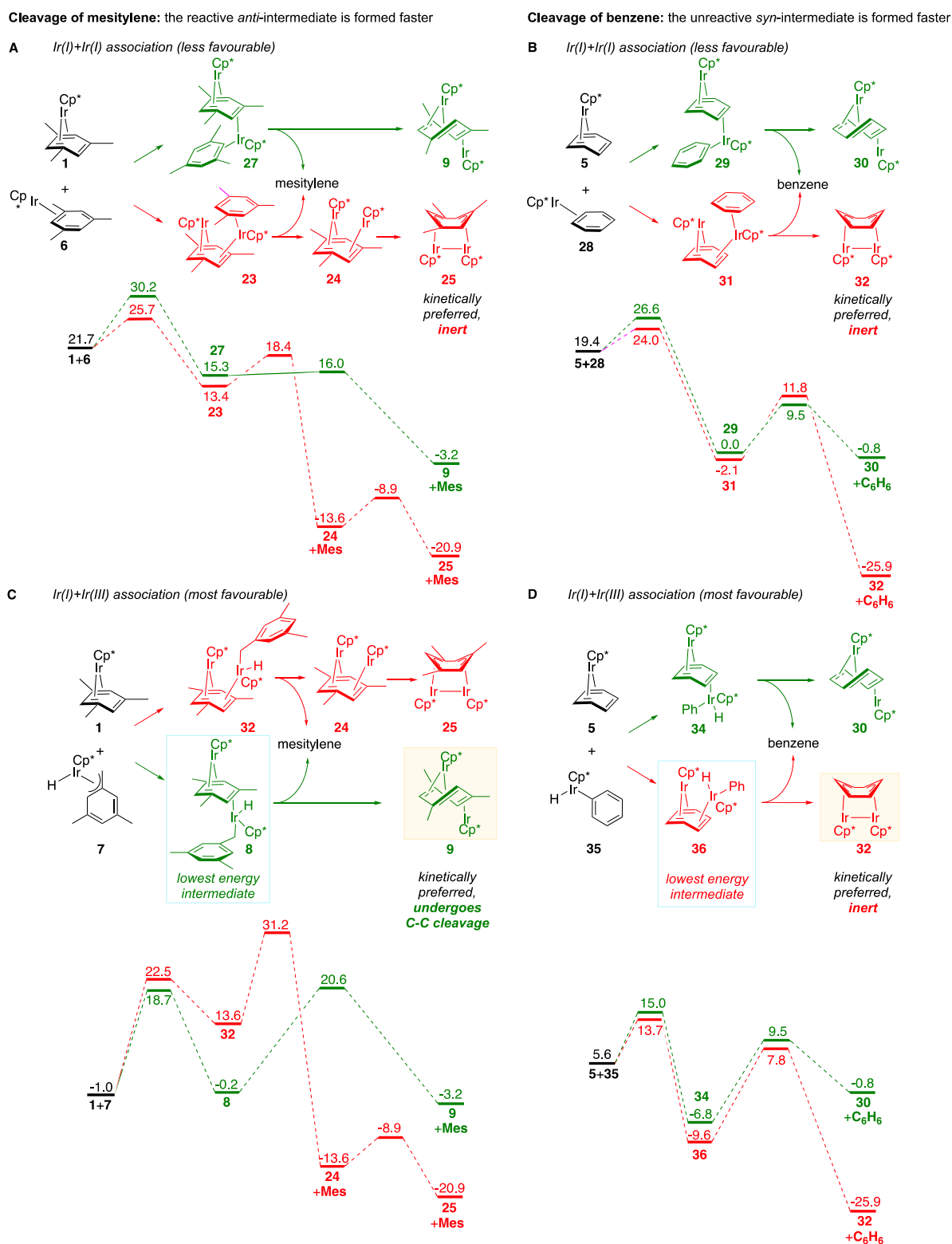
Figure 7. Calculated competing mechanisms of the formation of syn and anti diiridium intermediates by association of reactant \text{Cp}^*\text{Ir}(\eta^4\text{-arene}) with either \text{Ir}^{\text{I}} (A and B) or \text{Ir}^{\text{III}} (C and D) intermediate in thermolysis of \text{Cp}_2\text{Ir}(\eta^4\text{-mesitylene}) (A, C) or \text{Cp}_2\text{Ir}(\eta^4\text{-benzene}) (B, D). The free energies are relative to two moles of \text{Cp}^*\text{Ir}(\eta^4\text{-arene}) in all schemes. Pathways in green and red lead to the reactive and unreactive intermediates, respectively. The boxed structures are the predicted products. All free energies are at M06-L/(6-311+G(d)+LANL2TZ)//B3LYP/(6-31G(d)+LANL2DZ), 1 M concentrations and 50 °C, relative to 2 moles of 1 (A and C) or of \text{Cp}^*\text{Ir}(\eta^4\text{-C}_6\text{H}_6) (B, D).
