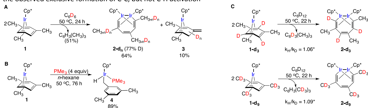
Figure 2. (A) H/D exchange and the formation of tautomer 3 upon heating 1 in C_6D_6 . (B) Benzylic C-H activation upon heating of 1 in the presence PMe_3 . (C) The lack of KIE and intramolecular H/D scrambling upon cleavage of 1-d 3 and 1-d 9 . *KIEs were calculated from initial rates for separate reactions of the deuterated and non-deuterated species.
