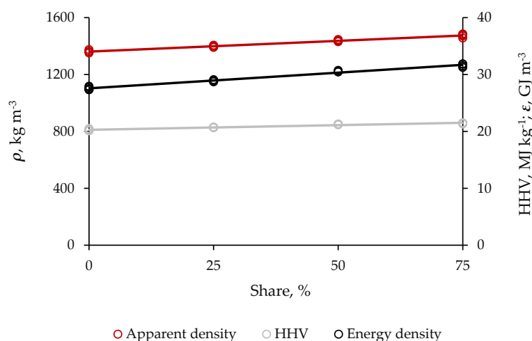
Figure 3. Effect of share of residual biomass from distillation of cellulosic bioethanol in the blend with sugarcane bagasse on the physicothermal quality of hybrid non-wood pellets. The steeper the line is, the larger the probability of the factor becoming the cause of significant variability is, as it gains in linearity; apparent density ( \rho ), higher heating value, (HHV) and energy density ( \epsilon ).
