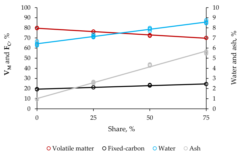
Figure 4. Effect of share of residual biomass from distillation of cellulosic bioethanol in the blend with sugarcane bagasse on the proximal properties of hybrid non-wood pellets. The steeper the line is, the larger the probability of the factor becoming the cause of significant variability is, as it gains in linearity; volatile matter ( V_M ) and fixed carbon ( F_C ).
