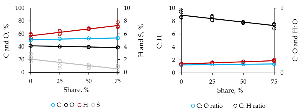
Figure 5. Effect of share of residual biomass from distillation of cellulosic bioethanol in the blend with sugarcane bagasse on the elemental properties of composite pellets. The steeper the line is, the larger the probability of the factor to becoming the cause of significant variability is, as it gains in linearity.
