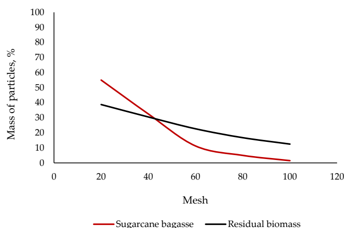
Figure 1. Distribution of particles' size of the ingredients for making hybrid non-wood pellets. The flatter the curve is, the more homogeneous the feedstock is, as it gains in regularity of size and shape of particles. The steeper the curve is, the greater the probability is that the material will become heterogenous, as the range of size of particles, from fine to coarse, is likely to be significantly large.
