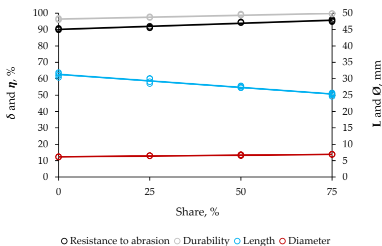
Figure 2. Effect of share of residual biomass from distillation of cellulosic bioethanol in the blend with sugarcane bagasse on the physicochemical quality of hybrid non-wood pellets. The steeper the line, the larger the probability of the factor to becoming the cause of significant variability, as it gains in linearity; length ( L ), diameter ( \emptyset ), durability ( \delta ), and resistance to abrasion ( \eta ).
