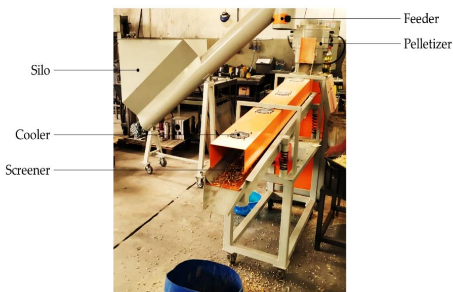
Figure 6. Pilot-scale integrated set for pelleting.
