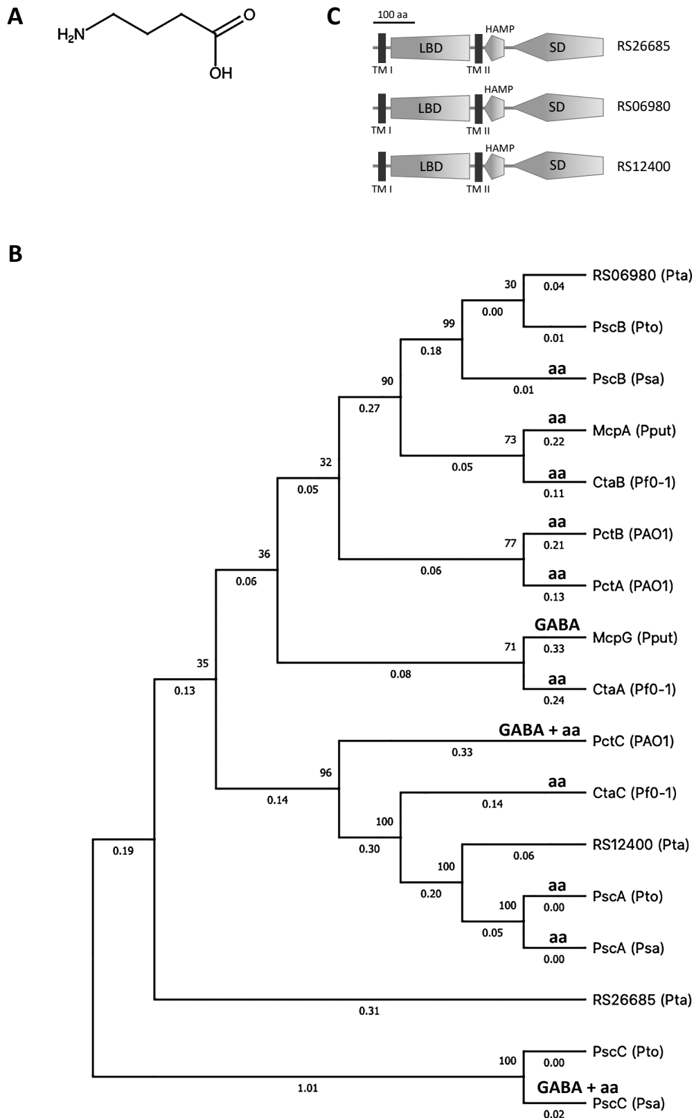
Fig. 1. GABA structure (A) and maximum likelihood tree based on ligand-binding domains (LBDs) of amino acid (aa) receptors and their homologs in Pseudomonas species (B). Phylogenetic tree of amino acid sequences of the LBD of McpG and McpA, a GABA and amino acid receptor of Pseudomonas putida KT2440; PctC, a GABA receptor and PctA and PctB, amino acid receptors of Pseudomonas aeruginosa PAO1; CtaABC, amino acid receptors of Pseudomonas fluorescens Pf0-1; PscABC, potential receptors for amino acids and GABA of Psa NZ-V13 and amino acid receptor and its paralog of Pto DC3000; RS26685, RS12400, and RS06980, predicted GABA and amino acid receptors of Pta6605 . Corresponding ligands are indicated by bold letters ( aa and GABA ). Branch length and bootstrap values are indicated on the tree. The tree was generated using MEGA version X software. Schematic structure of three MCP proteins of Pta6605 (C). Transmembrane domains (TMI and TMII), ligand-binding domains (LBD), h istidine kinase, a denyl cyclase, m ethyl-accepting chemotaxis proteins and p hosphatase (HAMP) domains, signaling domains (SD), and the scale of 100 amino acids are indicated.
