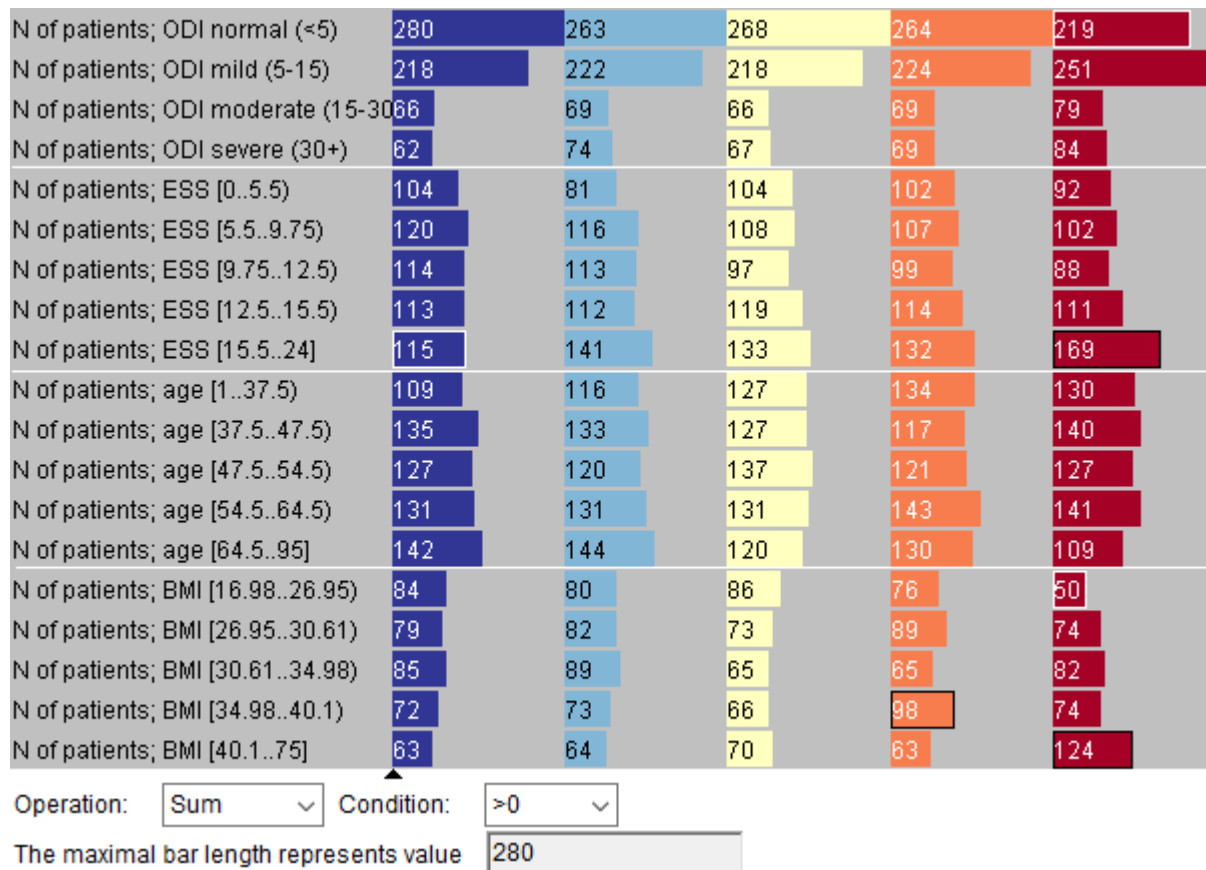
Figure 9. Counts of the patients by the area classes and value intervals of the attributes ODI (oxygen desaturation index), ESS (self-estimated sleepiness), age, and BMI (body mass index).
