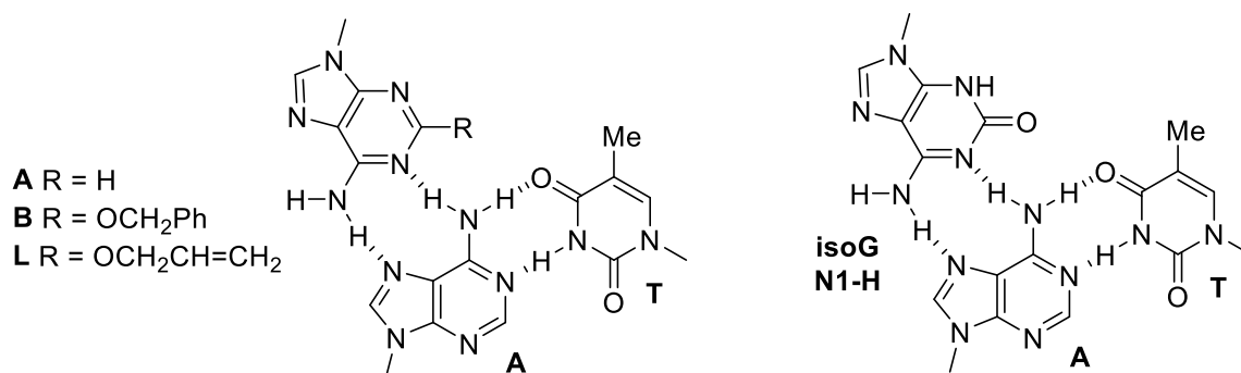
Figure 2. Triplex DNA motifs involving adenine ( A ) and the adenine-like 2-benzyloxyadenine ( B ), 2-allyloxyadenine ( L ) (left) and N1-H tautomer of isoguanine ( isoG ) (right).
