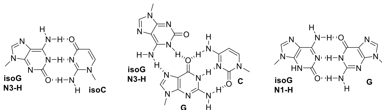
Figure 1. Representative motifs in oligonucleotides where the N3-H tautomer of isoguanine ( isoG ) is targeted to isocytosine 7 ( isoC ), to a guanine.cytosine ( G.C ) base pair 29 and as the N1-H tautomer, targeted to guanine 32 ( G ).
