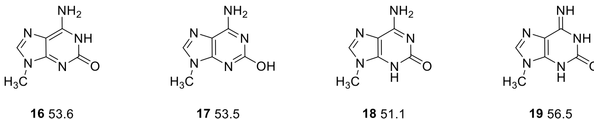
Figure 3. The calculated (AM1) heats of formation \Delta H_f (kcal.mol -1 ) for N9 methylated isoguanine tautomers 16 N3-H, 17 O2-H, 18 N1-H, and 19 6-imino-2-oxo.
