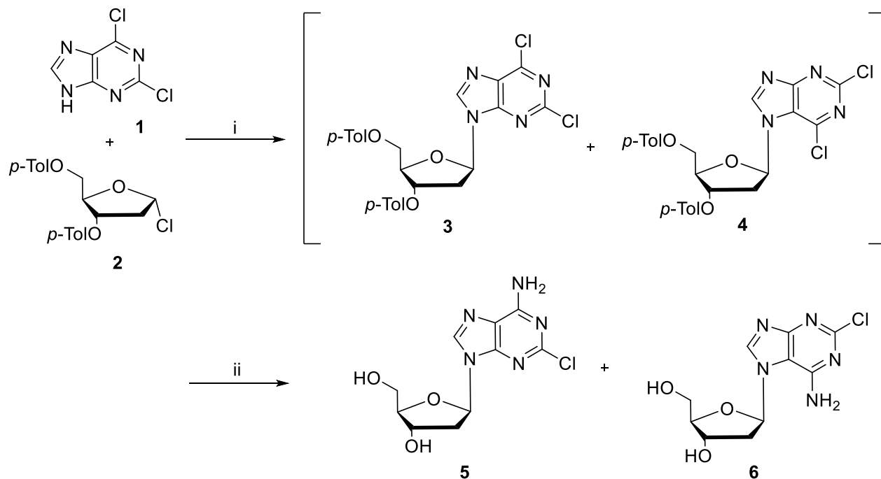
Scheme 1. Reagents and conditions: i, NaH, MeCN, rt, 24 h ; ii, MeOH-NH 3 (satd.), 100 °C, 6 h.
