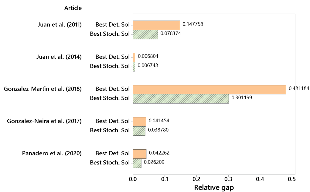
Figure 1: Relative gaps of the best stochastic and deterministic solutions found by simheuristics compared to the deterministic value of the best-known solutions.
