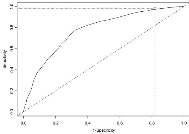
Receiver Operating Characteristic Curve for Scoring System
