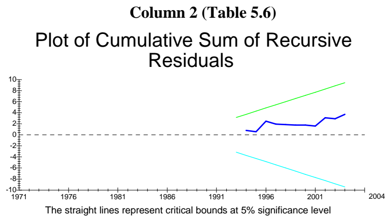
Figure 5.16: The Plot of CUSUM and CUSUM-Q tests
