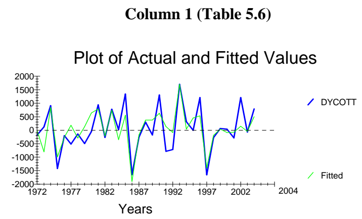
Figure 5.13: Plot of Actual and Fitted Values of Residual
