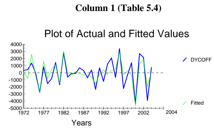
Figure 5.11: Plot of Actual and Fitted Values of Residual
