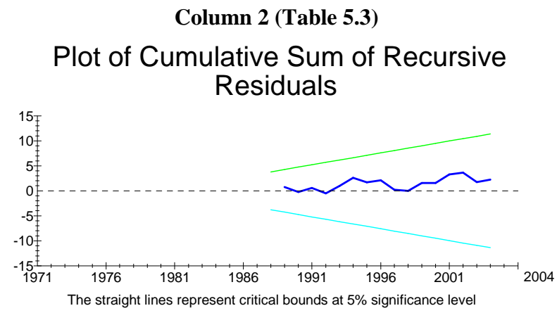
Figure 5.14: The Plot of CUSUM and CUSUM-Q tests
