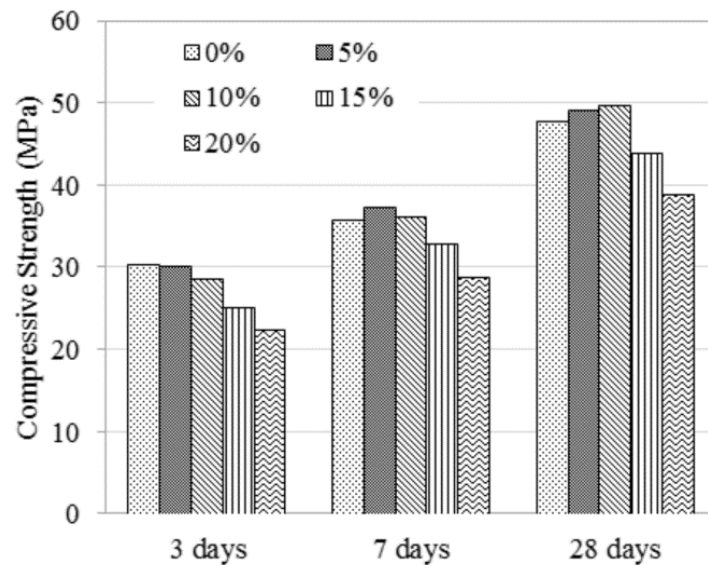
Fig. 3 Type IP cement with limestone fines mortar compressive strength.
