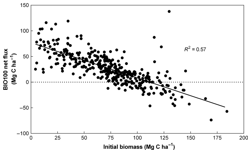
Fig. 6 Linear regression of net flux from BIO100 scenario and starting live biomass. Y = -0.6891 \cdot X + 77.01 .
