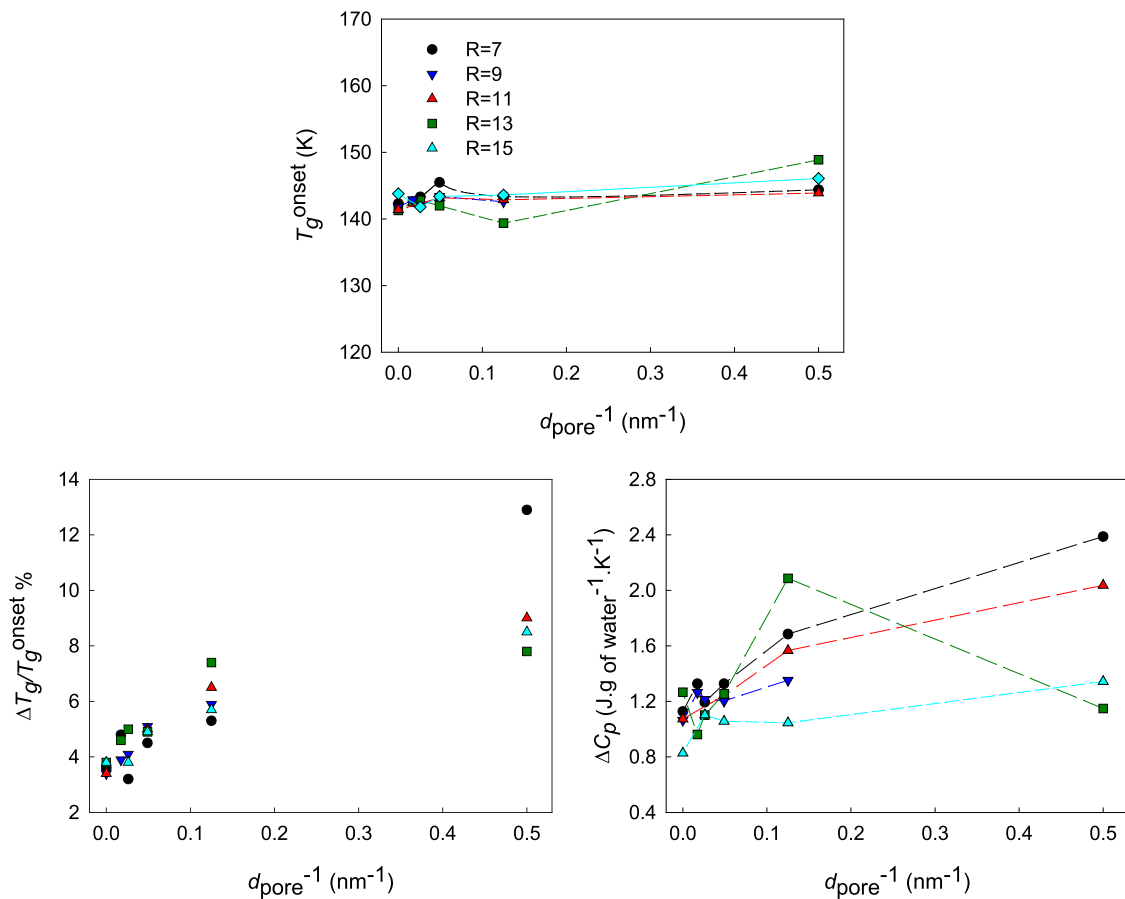
FIG. 5. Onset glass transition temperatures T_{g,onset} , width of the glass transition 100 \Delta T_g / T_{g,onset} , and change of heat capacity \Delta C_p for the glass transition for all LiCl aqueous solutions studied in this work plotted against inverse pore diameter.
