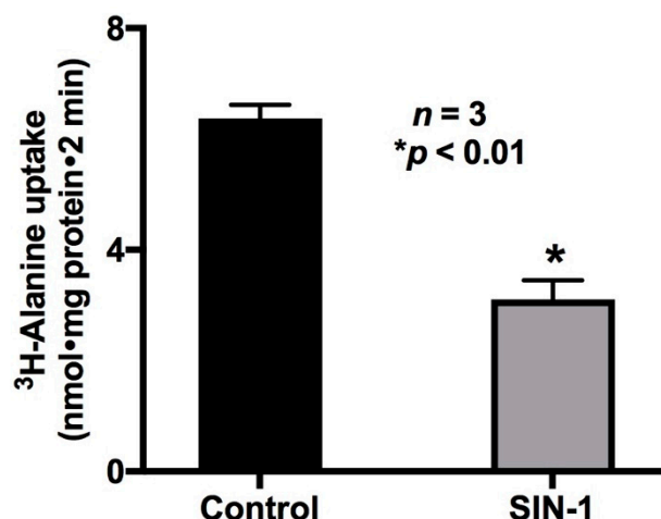
Figure 1. Effect of peroxynitrite (OONO) on Na-alanine co-transport (ASCT1) in IEC-18 cells. Na-stimulated ^3\text{H} -alanine uptake was reduced in SIN-1-treated cells. Thus, OONO inhibits Na-alanine co-transport in IEC-18 cells.
