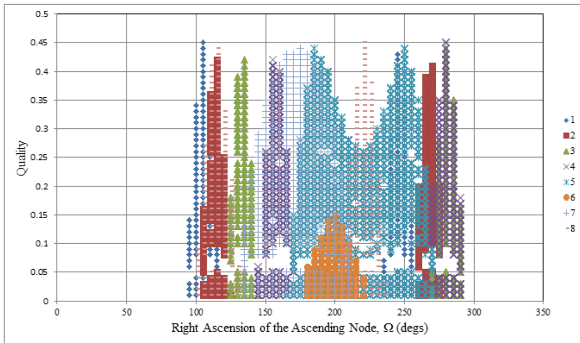
Figure 60 Right Ascension of Ascending Node vs. Total Quality for Multiple Headings at V_f=0.1
