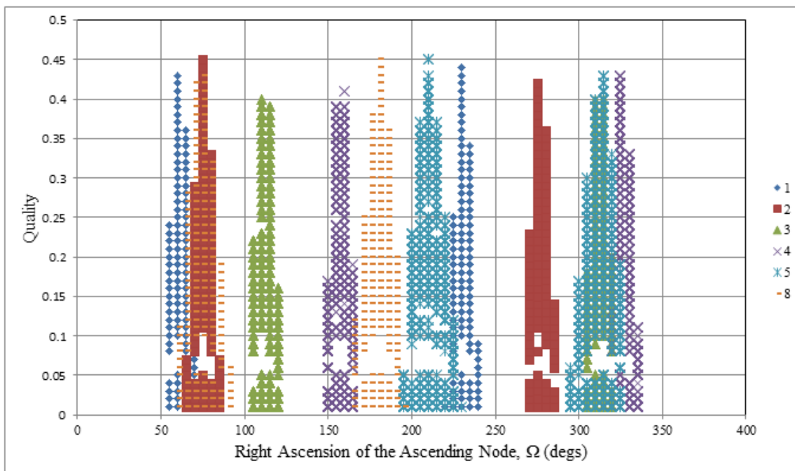
Figure 63 Right Ascension of Ascending Node vs. Total Quality for Multiple Headings at V_f=0.4
