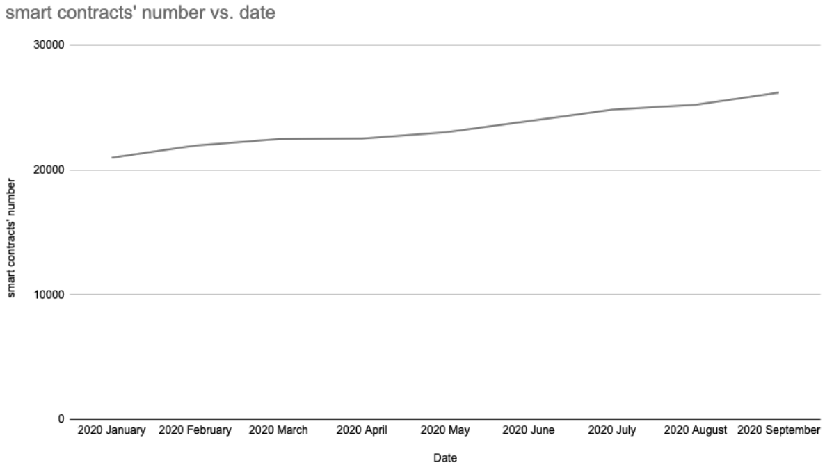
Fig. 7: Number of smart-contracts' collected in Smart Corpus.
