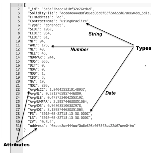
Fig. 3: Smart-Corpus's database schema
