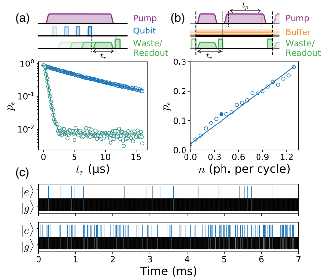
FIG. 3. Reset protocol and cyclic operation. (a) The qubit is initialized in its excited state (blue pulse) and the pump is activated. The decay of p_e is measured (open circles) in the presence (green) or absence (blue) of a reset tone of duration t_r applied to the waste mode (green pulse). The exponential fits (solid lines) yield a qubit T_1 reduced from 7.7 \mu\text{s} to 370 \text{ ns} . Note that the residual qubit population is reduced in the presence of the reset tone from 3.5\% (see Fig. 2) to 0.7\% , demonstrating that the reset is in fact cooling the qubit below its effective bath occupation. (b) Cyclic operation of the pulse sequence in between the two vertical dashed lines, in the presence of a continuous input tone of variable amplitude (orange pulse). First, the qubit is reset for 2 \mu\text{s} (first green and purple pulses), followed by a heralding measurement to confirm the preparation in the ground state (second green pulse). The detector is then activated during a time t_p = 3 \mu\text{s} by switching on the pump (second purple pulse), and finally, the qubit state is read out (third green pulse). The measured p_e (open circles) is plotted as a function of the photon number in the input pulse integrated over the cycle time 7 \mu\text{s} . A linear regression (solid line) yields an overall efficiency of 20\% (which accounts for the 43\% duty cycle) and a dark count of 2\% per cycle. (c) Real-time trajectories of 1000 successive detection cycles, with \bar{n} = 0 (top) and \bar{n} = 0.38 (bottom), as marked by the full dot in (b).
