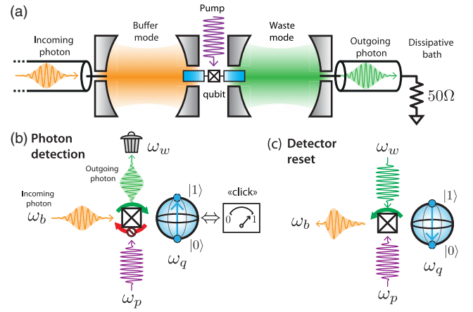
FIG. 1. Principle of the itinerant photon detector. (a) The circuit consists of two microwave modes: a buffer (orange) and a waste (green) coupled to a transmon qubit (blue). Each mode is well coupled to its own transmission line so that a photon can enter the device on the left and leave on the right into the dissipative 50\ \Omega environment. A pump (purple) is applied on the Josephson junction to make the three-wave mixing interaction resonant [Eq. (2)]. (b) When a photon enters the buffer, the pump converts it via the Josephson nonlinearity (black cross) into one excitation of the qubit and one photon in the waste. The waste excitation is irreversibly radiated away in the transmission line, so that the reverse three-wave process cannot occur. The quantum state of the qubit is measured with a standard dispersive readout via the waste to detect whether or not a photon arrived while the pump was on. (c) When a coherent tone drives the waste, the qubit excitation can combine with waste photons and be released via the Josephson nonlinearity in the buffer, enabling a fast reset of the detector.
