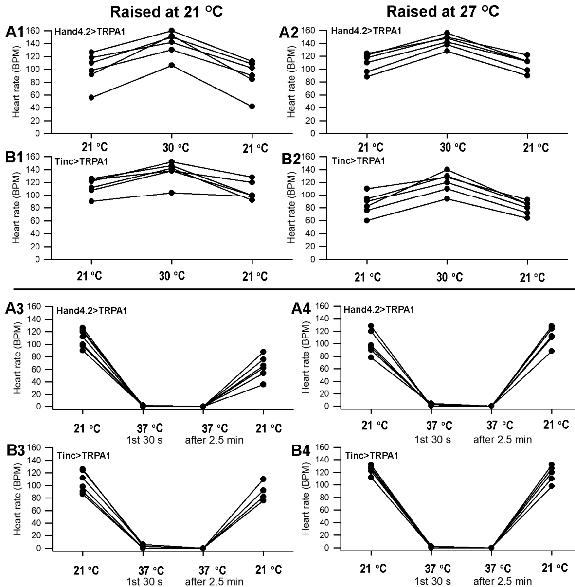
Figure 5. The heart rate for the dissected larvae over-expressing TrpA1 specifically in the heart. The heart rate increased in Hand4.2>TrpA1 (A1,A2) and Tinc>TrpA1 (B1,B2) from 21 to 30 °C ( p < 0.05 , paired t -test) for both conditions of larvae raised at 21 °C (A1,B1) as well as at 27 °C (A2,B2). The strains Hand4.2>TrpA1 (A3,A4) and Tinc>TrpA1 (B3,B4) upon exposure at 37 °C all rapidly decreased heart rate and maintained a low rate for 2.5 min. Upon exposure to 21 °C, the rates increased. The same trend was present for the larvae raised at 21 °C (A3,B3) as well as at 27 °C (A4,B4). Controls for these strains are illustrated in Figure 4 top panels under the same conditions.
