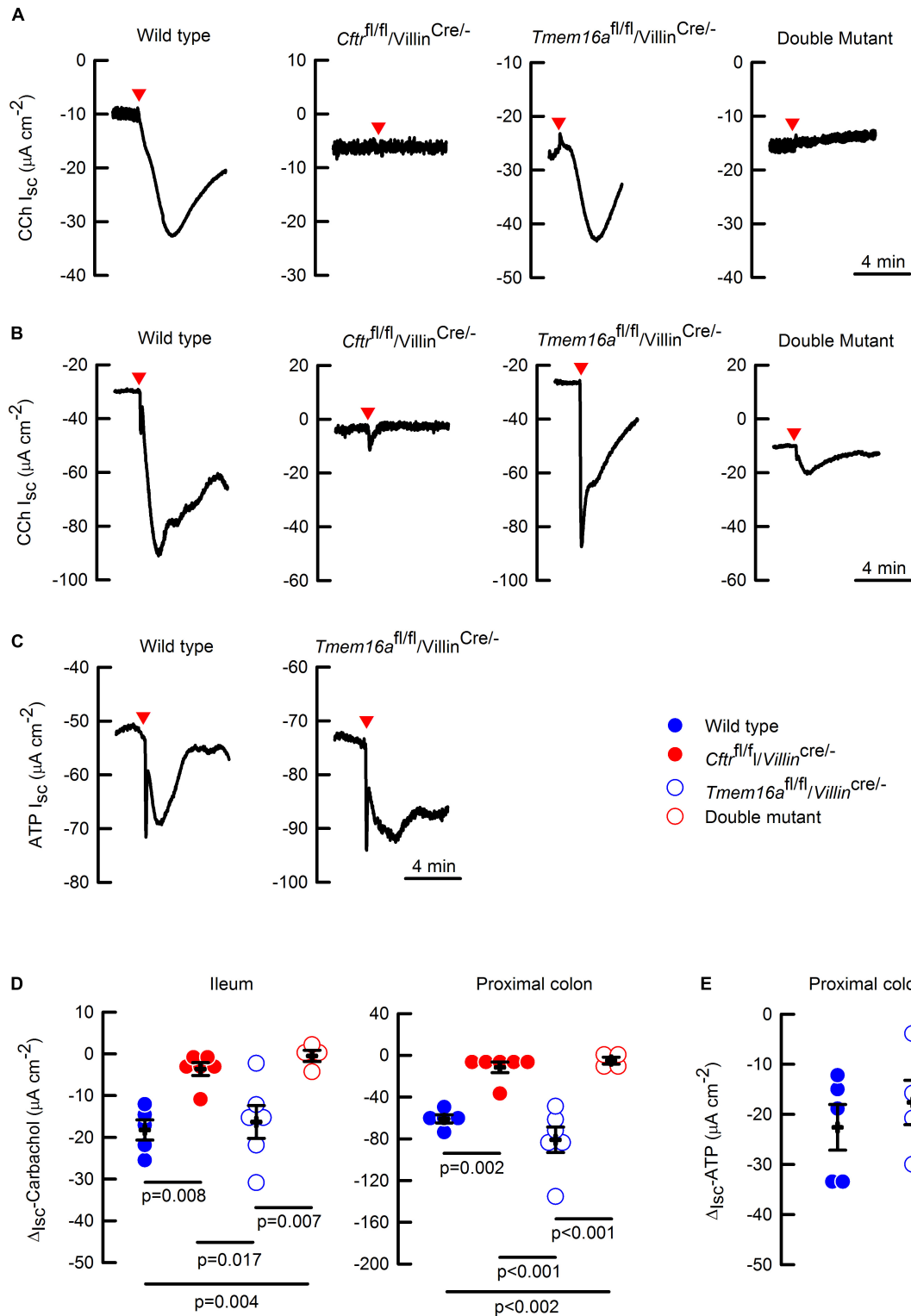
FIGURE 3 | Cftr but not Tmem16a silencing abolished calcium-activated anion secretion in mouse intestine. Representative images of CCh-induced short-circuit currents ( I_{sc} ) from in the ileum (A) and proximal colon (B) of the different mice. (C) Representative images of ATP-induced short-circuit currents in the wild type and Tmem16a fl/fl / Villin Cre/- mice. Red arrowheads indicate the time of CCh (100 \mu M ) or ATP (100 \mu M ) addition on the basolateral side for each image. Short-circuit current changes ( \Delta I_{sc} ) in ileum and colon induced by CCh (D) , and in colon induced by ATP (E) , are summarized; n = 4-6 for CCh in ileum and colon on each group; n = 5 for wild type and n = 4 for Tmem16a fl/fl / Villin Cre/- in the ATP experiments. Indicated p values correspond to one way ANOVA (D) or unpaired t -test (E) analysis. No significant difference found for groups in panel (E) .
