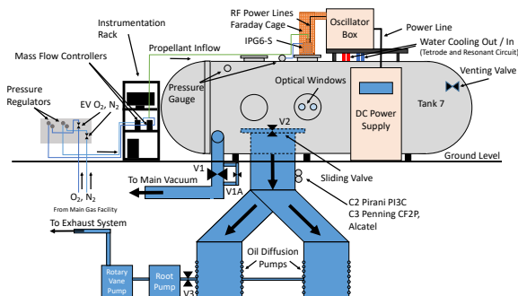
Figure 7 IPG6-S Facility Set-Up
