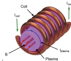
Figure 2 IPG Principle of operation [3]
