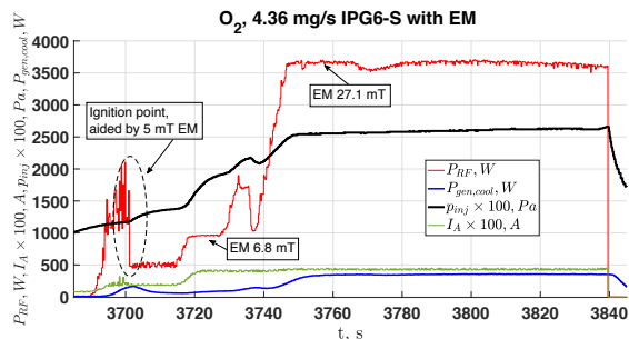
Figure 9 O_2 Test, effect of applied magnetic field
