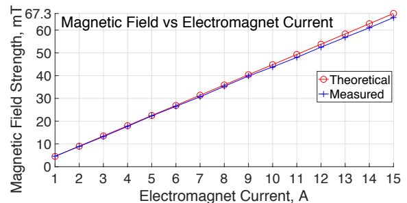
Figure 4 Electromagnet Performance, measured and theoretical.
