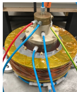
Figure 6 IPG6-S with EM installed
