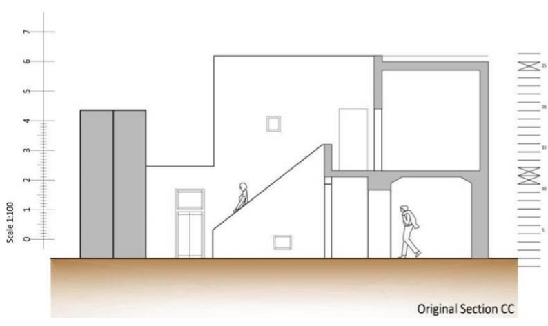
Figure 4.9: Sections corresponding to layout plans (Wismayer, 2013)
