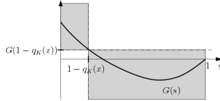
Figure 1-4: Graph of the branching generator G split at 1 - q_K(x) ; rescaling the upper-left quadrant and lower-right quadrant gives the branching generators G^R and G^B respectively.
