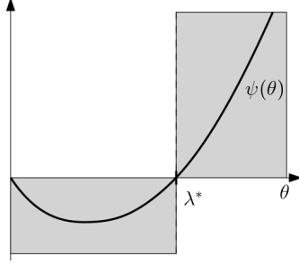
Figure 1-5: Graph of the branching mechanism \psi split at \lambda^* ; rescaling the lower-left quadrant and upper-right quadrant gives the branching generator F and branching mechanism \psi^* respectively.
