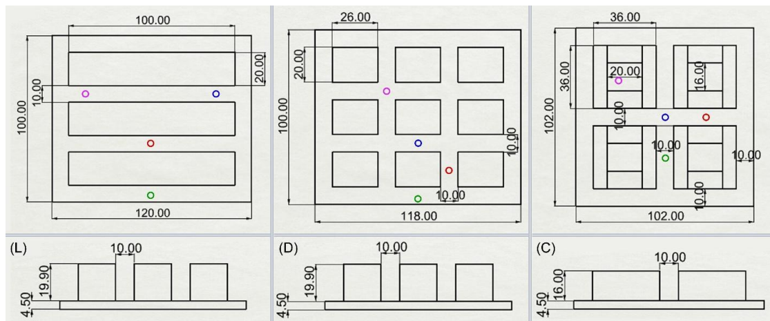
Figure 1: Geometry configurations for the three layouts; (L) Linear; (D) Dotted; and (C) Courtyard (dimensions in meters). Coloured circles denote to (Green) Receptor R1, (Red) R2, (Blue) R3, and (Purple) R4.
