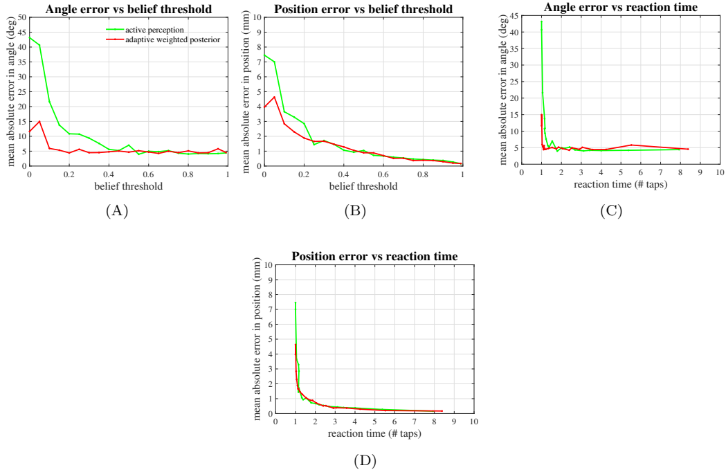
Figure 8: Adaptive weighted posterior strategy employed with active perception for recognition of angle and position perceptual classes during a contour following exploration procedure (red colour curves). (A) High angle recognition accuracy is achieved with small belief threshold values. (C) Reaction time is also improved requiring less number of tactile contacts to make a decision. These results improve the performance of active perception alone. (B) Recognition of position classes shows slight improvement for small belief thresholds. (D) However, reaction time for recognition of position classes does not show improvement. Results from the use of active Bayesian perception alone are also included (green color curves) for comparison of performance.
