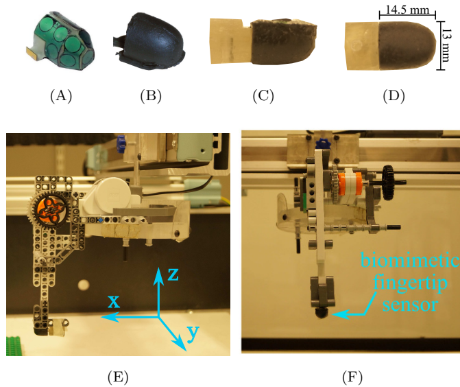
Figure 1: Tactile sensory system and exploratory robotic platform. (A) Flexible PCB and taxels of the iCub fingertip. (B) Fingertip sensor covered with dielectric silicon. (C) Lateral view of the sensor. (D) Dimensions of the biomimetic sensor. (E),(F) Robotic platform for tactile exploration in x -, y - and z -axes.
