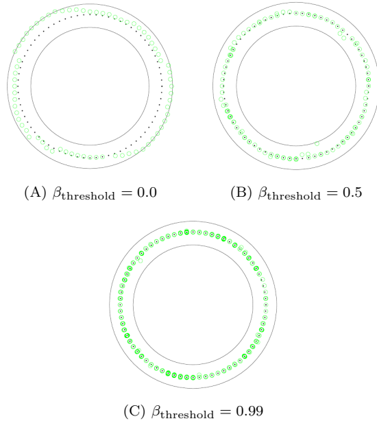
Figure 6: Tactile contour following results from a circular-shaped object using active perception and a biomimetic fingertip sensor. The object contour is defined by the black dotted line, sensor movements are represented by the green colour circles and the black solid line defines the exploration limits according to the collected datasets. (A) Active perception with belief threshold, \beta_{\text{threshold}} = 0.0 , does not allow the touch sensor to extract the object shape. (B) Active perception with belief threshold, \beta_{\text{threshold}} = 0.5 , improves the exploration process but still the object shape is not extracted successfully. (C) Large belief thresholds, \beta_{\text{threshold}} = 0.99 , allow the active perception approach to successfully follow and extract the object shape.
