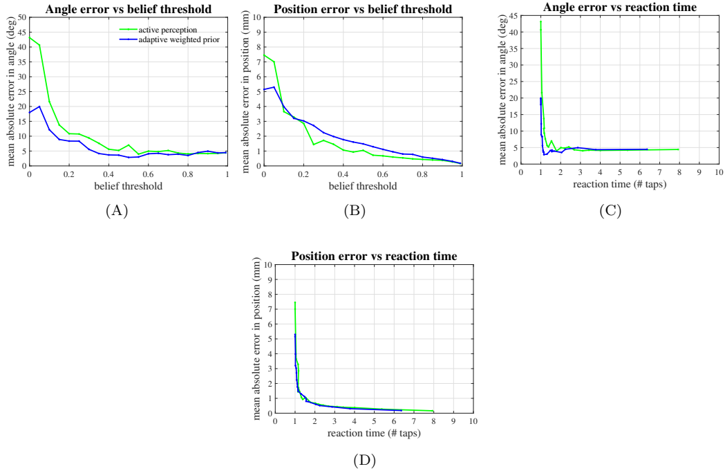
Figure 7: Adaptive weighted prior strategy employed with active perception for recognition of angle and position perceptual classes during a contour following exploration procedure (blue colour curves). (A) Angle perception accuracy is improved requiring small belief threshold values to achieve high accuracy. (C) This result also improves the reaction time for angle perception. (B,D) Recognition of position classes and reaction time do not show improvement by the adaptive weighted prior strategy. Results from the use of active Bayesian perception alone are included (green color curves) for comparison of performance.
