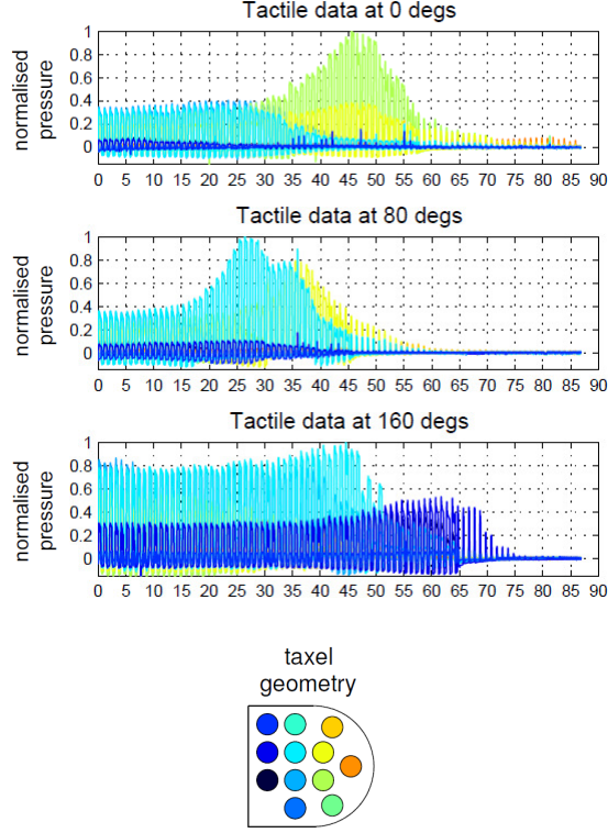
Figure 3: Sample of data collected with the biomimetic fingertip sensor. Datasets for orientation of the fingertip sensor at 0 deg, 80 deg and 160 deg along 18 mm (90 taps) over the plastic object used as stimuli. Normalised pressure measurements from activated taxels are shown by a coloured code.
