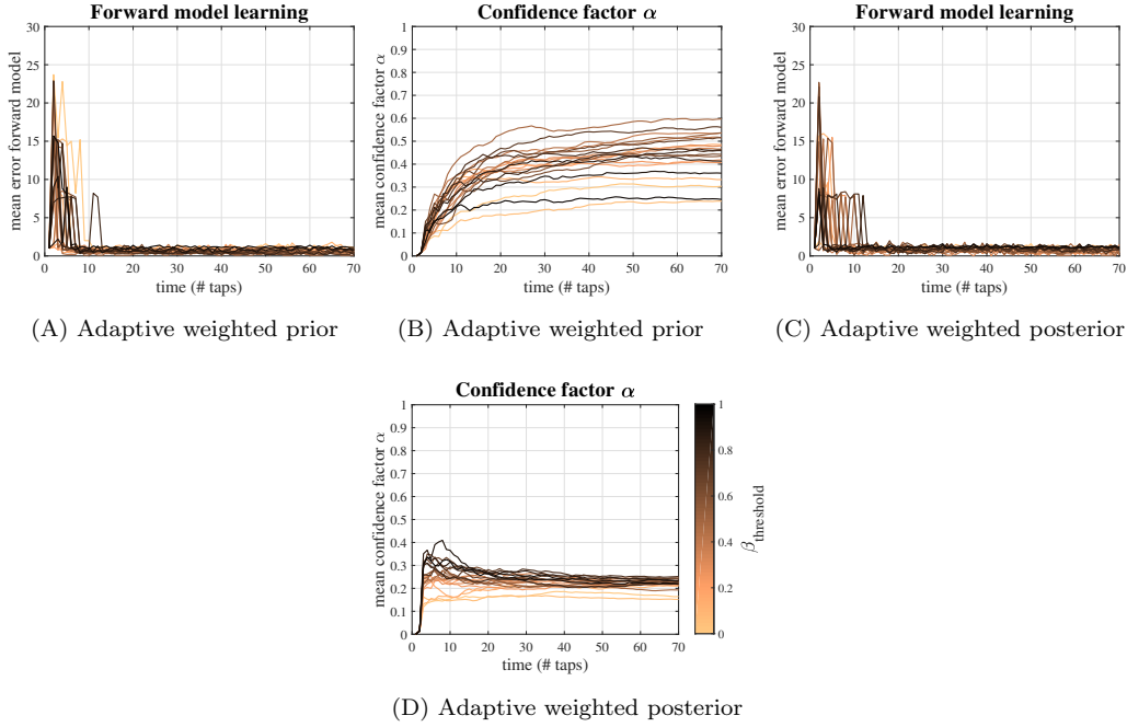
Figure 9: Forward model and confidence parameter implemented by the proposed adaptive strategies. These results are obtained from a contour following exploration procedure using a biomimetic fingertip sensor and evaluated with a set of belief threshold \beta_{\text{threshold}} = \{0, 0.05, \dots, 0.99\} , which are represented by coloured curves. (A) Adaptive weighted prior strategy; accuracy of the forward model for prediction of sensory observations improves over time. (B) Confidence parameter adapts over time, based on the accuracy of predictions, to control the combination of information sources by the adaptive weighted prior strategy. (C) Adaptive weighted posterior strategy; forward model accuracy improves over time. (D) Adaptive confidence parameter, based on the accuracy of prediction, which permit to control the combination of information sources by the weighted posterior strategy.
