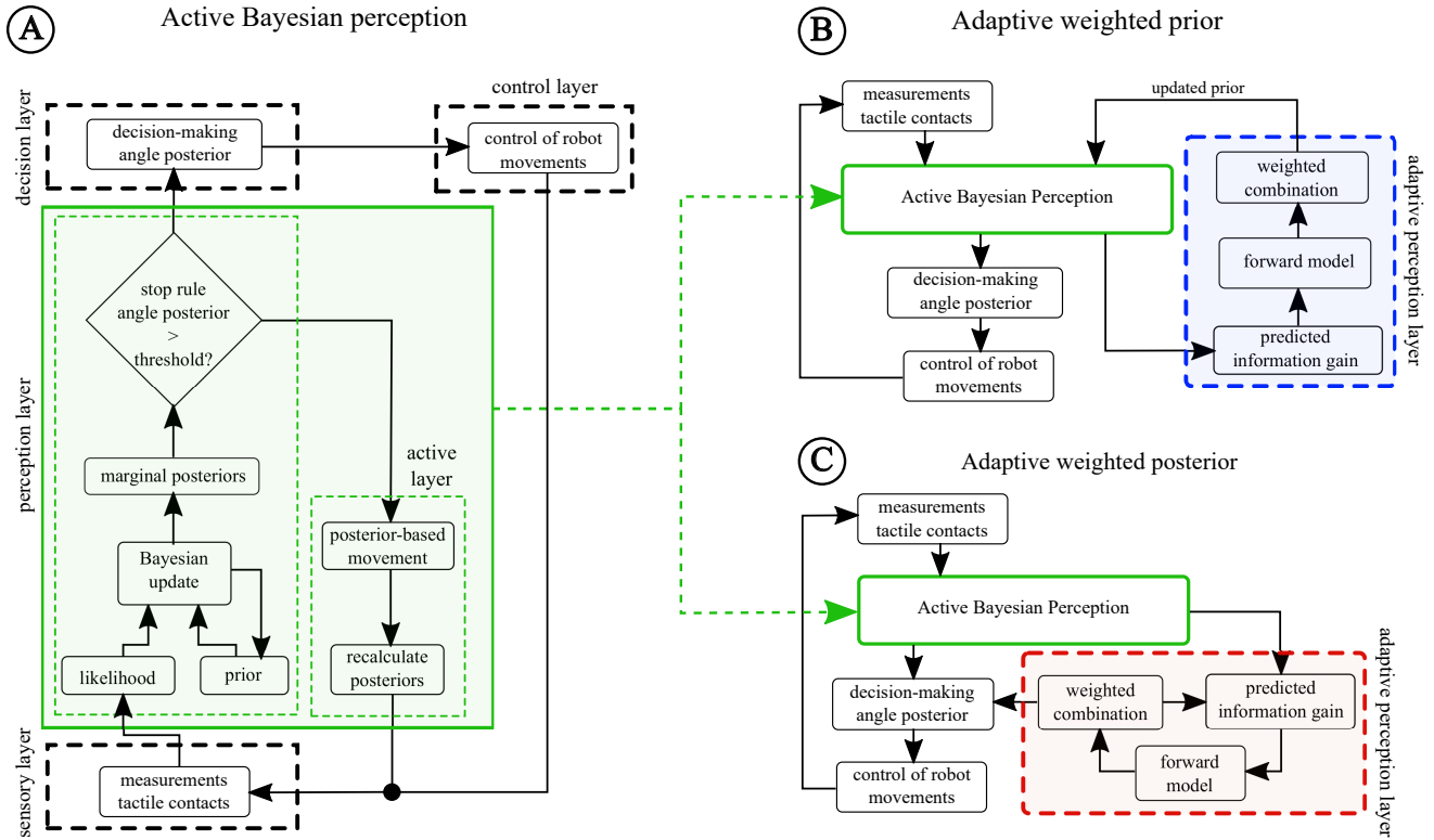
Figure 4: Flowcharts for active perception and adaptive strategies. (A) Active Bayesian perception composed of five layers: sensory , decision , control (black colour boxes), perception and active (green colour boxes). Perception layer accumulates evidence while actively reposition of the sensor by the active layer. Decision-making, by the decision layer, controls the movements of the robot platform in the control layer. (B) Adaptive weighted prior strategy (blue colour box) extends the active Bayesian perception (green colour box) using sensory predictions and combining them with current observations. This strategy, applied at the beginning of the perception process, impacts on the prior probability. (C) Adaptive weighted posterior (red colour box) allows the active perception to make sensory predictions and combine information streams, but in this case, this strategy takes place at the end of the perception process, impacting the posterior probability.
