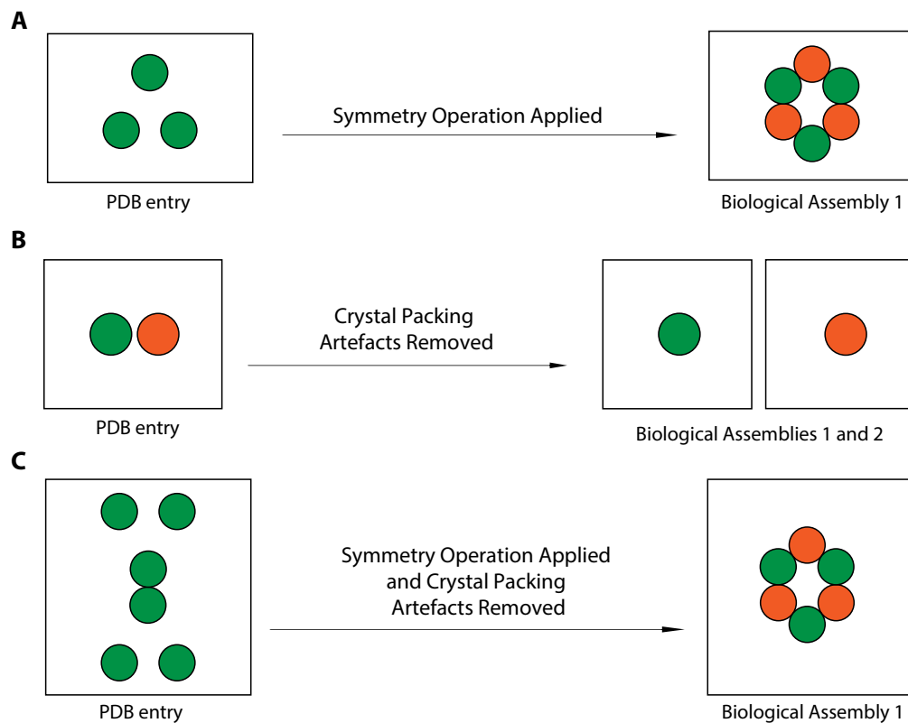
Figure 1.3: Generating biological assemblies from the asymmetric unit by applying biologically relevant symmetry operations and/or by removing crystal packing artefacts. Examples provided depict: A) generation of a biological assembly (BioUnit) by applying symmetry operations to the asymmetric unit (AsymUnit); B) generation of two BioUnits by removing crystal packing artefact interactions, and; C) generating a BioUnit by applying symmetry operations and simultaneously removing artefact crystal packing. Figure adapted from Jefferson et al., 2006.
