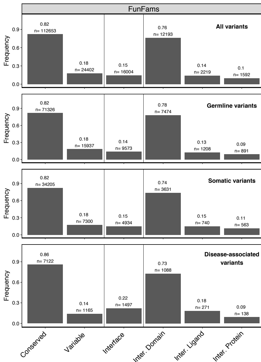
Figure 5.4: Distribution of genetic variants mapped to structurally conserved regions within interaction interfaces in FunFam domain families. Genetic variants were grouped as germline variants, somatic mutations and disease-associated variants. The aggregation of all variants in the three classes is also provided. n corresponds to the total number of genetic variants in each class that fall into that particular structure environment. Structural environments/regions were defined as described in Section 4.3.2. The number of variants in variable regions is shown for comparison purposes.
