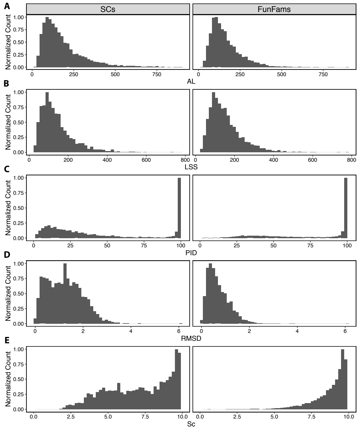
Figure 3.4: Overview of various STAMP alignment metrics for the comparison between SCs and FunFams. Histograms are provided for comparing: A) alignment length (AL); B) the length of the shortest domain sequence (LSS); C) the smallest percentage sequence identity (PID) observed; D) the Root Mean Square Deviation (RMSD); and E) STAMP Sc scores. Histogram binning was performed using normalised counts. The number of SCs and FunFams is 2,371 and 5,777, respectively.
