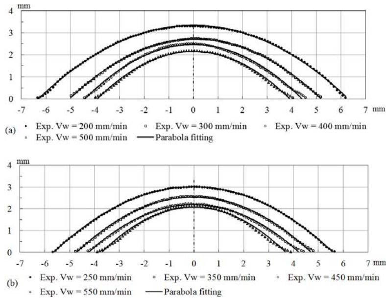
Fig. 4 Weld bead geometry of a single bead with various welding speeds
