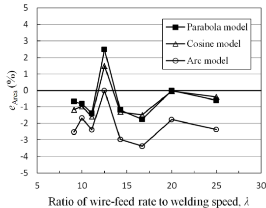
Fig. 3 Relative error for predicted and actual area of weld bead cross-section
