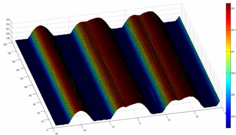
Fig.2 Experimental measurements of weld bead profile
