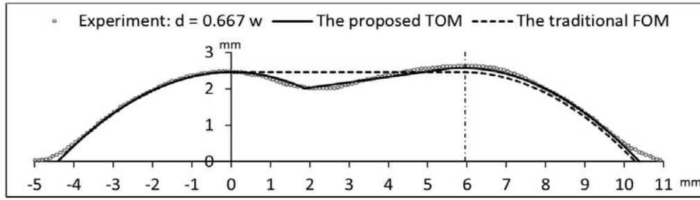
Fig.9 Comparison of experimental measurements of bead profile with the tangent overlapping model (TOM) and the flat-top overlapping model (FOM)
