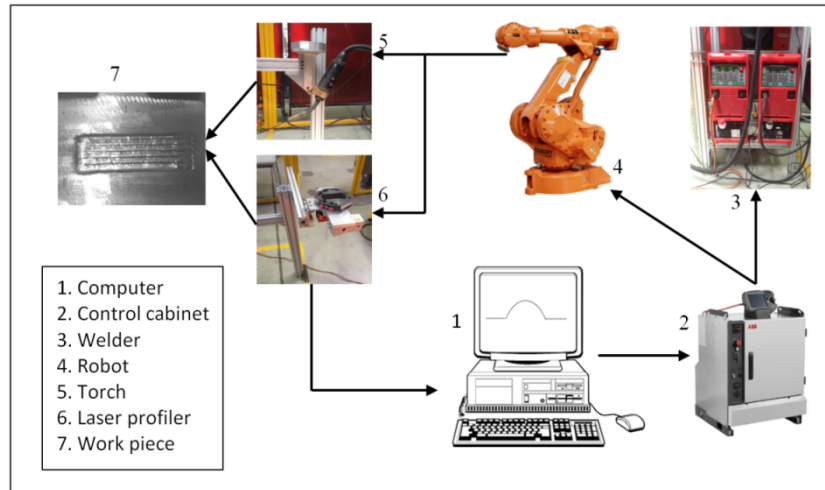
Fig.1 Schematic diagram of the experimental WAALM system
