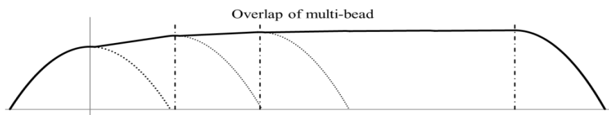
Fig.8 The schematic overlapped profile of a multi-bead deposit at d < d^*
