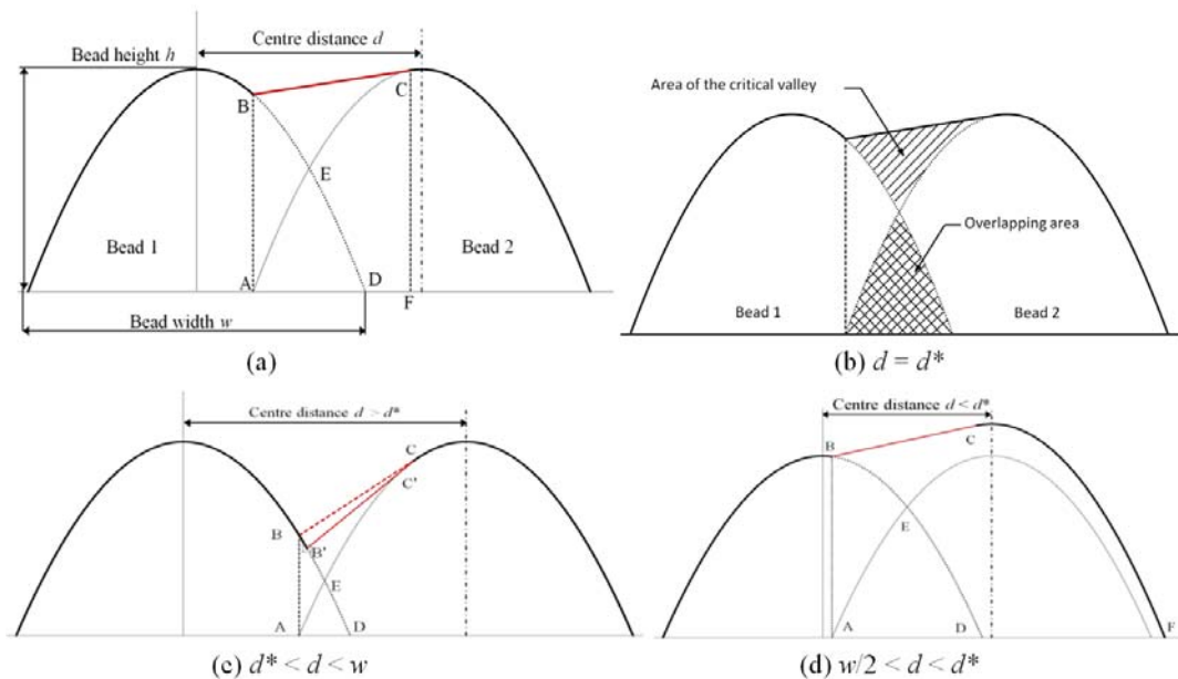
Fig. 6 Schematic diagrams of the tangent overlapping model (TOM)
