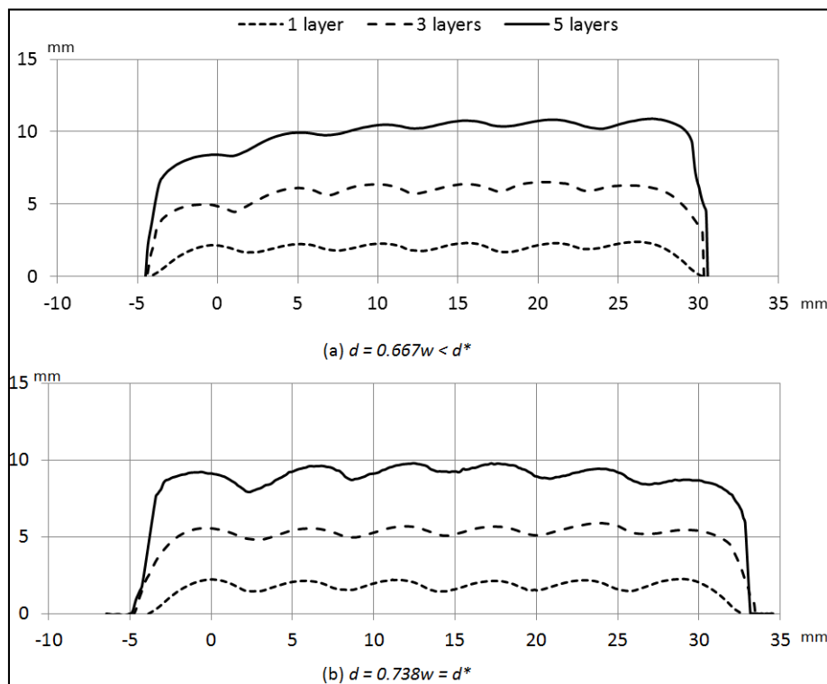
Fig. 13 Experiments of multi-bead and multi-layer deposition.
