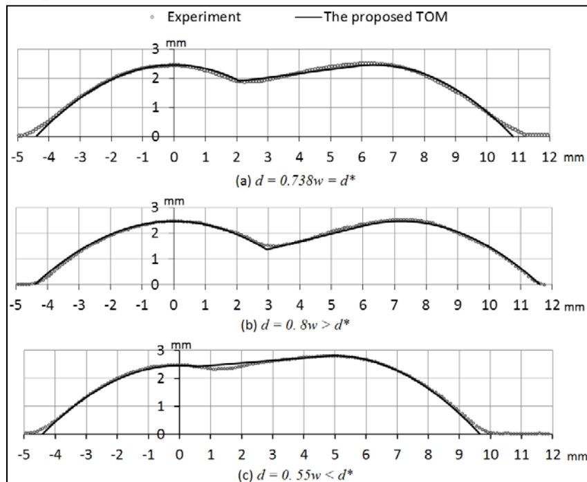
Fig. 11 The experimental results of overlapped bead profile at various centre distance d
