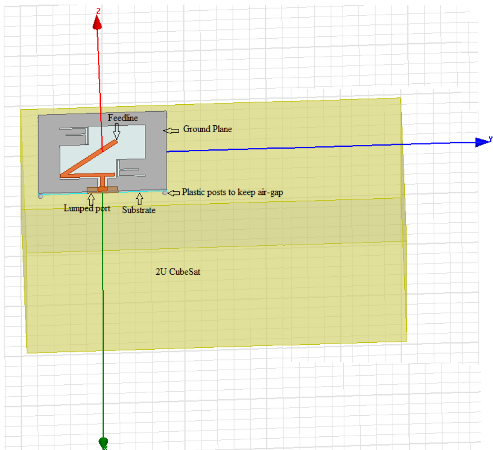
Figure 3. Geometry of CPW-feed square slot antenna on 2U CubeSat body
