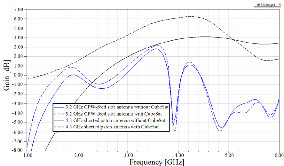
Figure 5. The simulated 2D gain of shorted patch and CPW-feed slot antenna with and without CubeSat body
