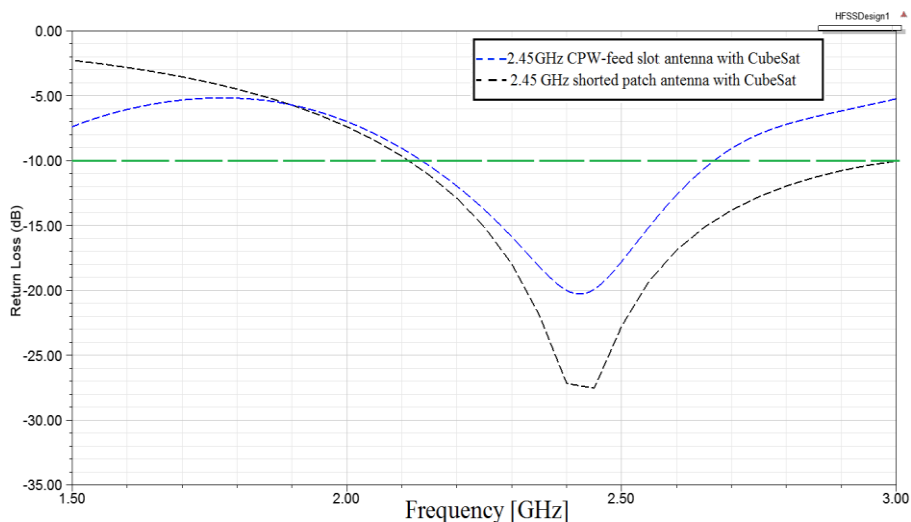
Figure 6. Simulated return losses of re-dimensioned shorted patch and CPW-fed slot antennas on 2U CubeSat
