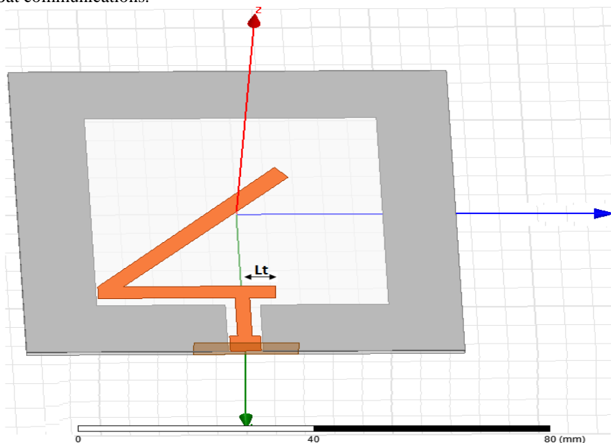
Figure 8. Geometry of re-dimensioned CPW-feed square slot antenna without F-shaped slits
