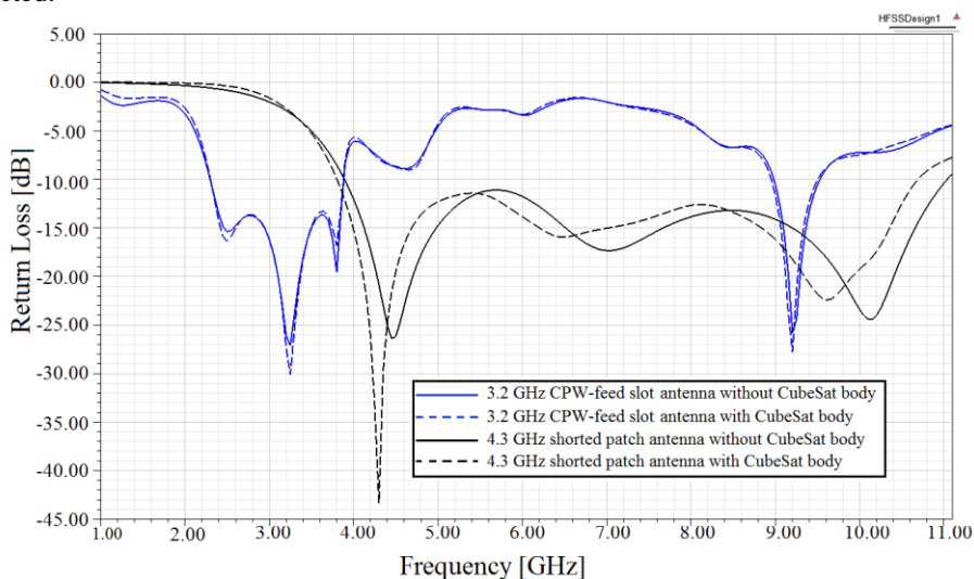
Figure 4. The simulated return loss of shorted patch and CPW-feed square slot antennas with and without CubeSat
