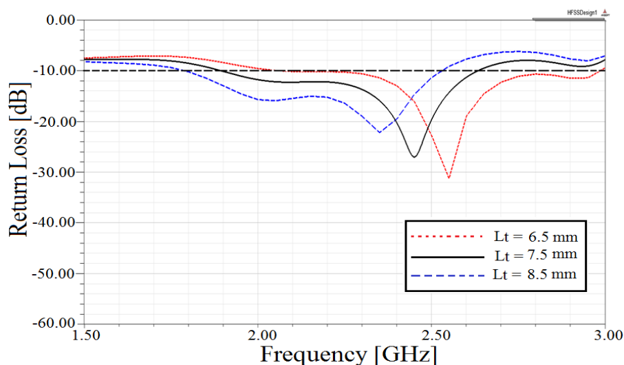
Figure 10. Simulated return loss against frequency for the various L_t
