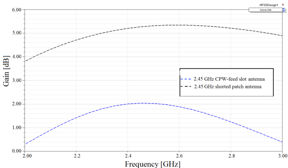
Figure 7. The simulated 2D gain of the modified shorted patch and CPW-feed slot antenna
