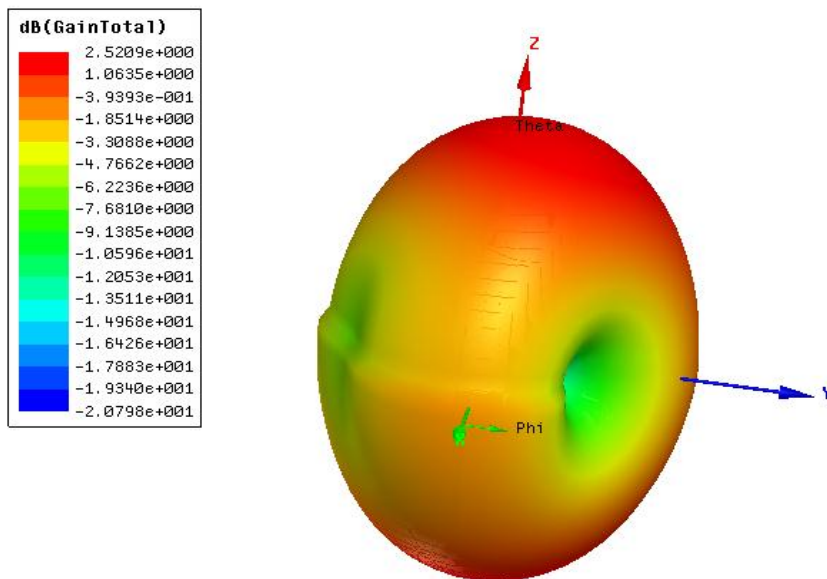
Figure 9. Total 3D gain of re-dimensioned CPW-feed square slot antenna after removing F-shaped slits
