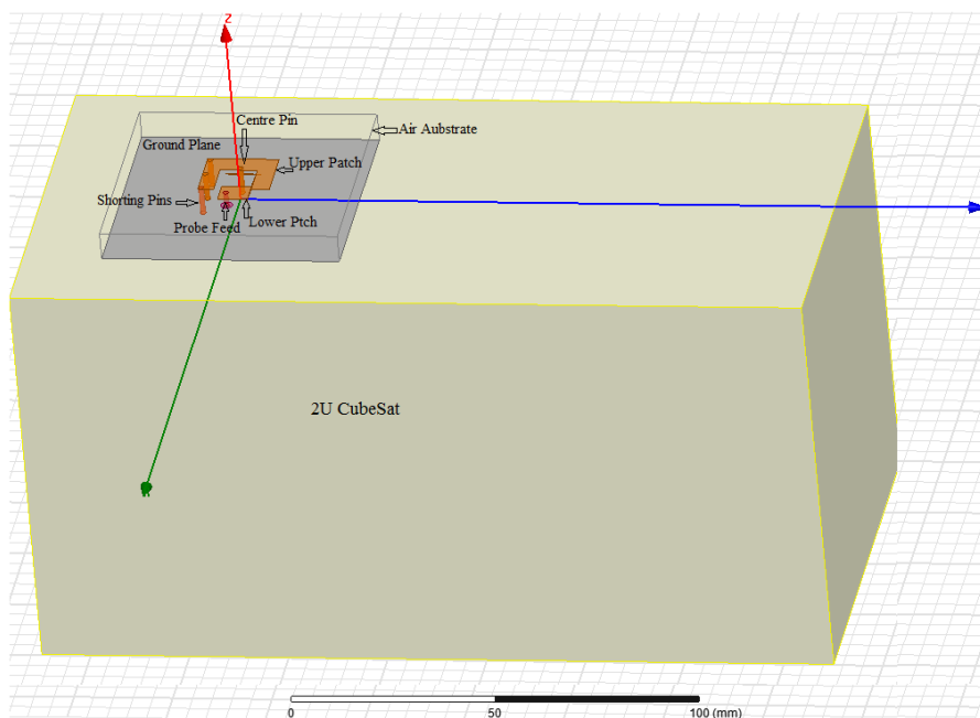
Figure 2. Geometry of shorted patch antenna on 2U CubeSat body
