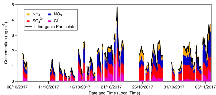
Figure 13. Summed mass and speciation of inorganic particulate recorded by GRAEGOR at 80 m throughout period of campaign.
