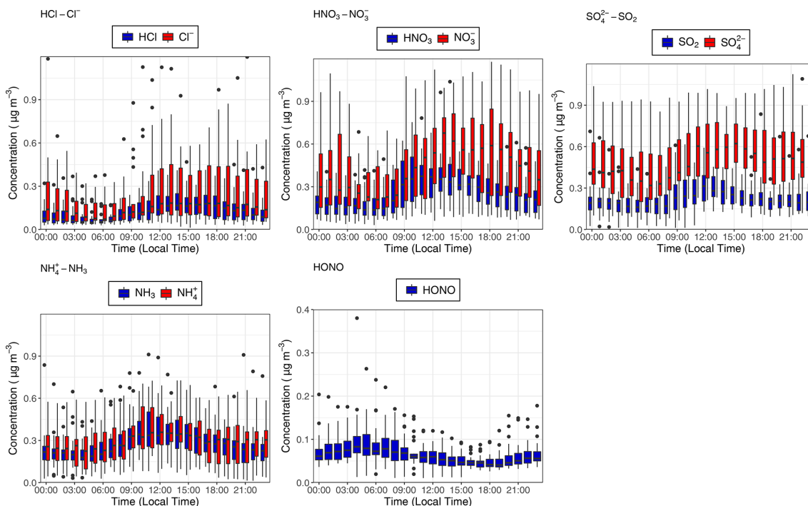
Figure 4. Median hourly diel concentrations for the inorganic trace gases \text{NH}_3 , \text{SO}_2 , \text{HONO} , \text{HNO}_3 and \text{HCl} in blue, as well as their paired associated aerosol counterparts \text{NH}_4^+ , \text{SO}_4^{2-} , \text{NO}_3^- and \text{Cl}^- in red at the 60 m sampling height measured during the campaign. The lower and upper edges of each box correspond to the first and third quartiles, respectively, while the whiskers extend to the largest and smallest values which do not exceed 1.5 times the inter-quartile range from their respective hinge. Black dots outside the plots are values which exceed 1.5 times the inter-quartile range.
