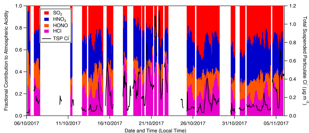
Figure 10. Fractional contribution to total measured inorganic acidity from \text{SO}_2 , \text{HNO}_3 , \text{HONO} and \text{HCl} as measured by GRAEGOR at 60 m (hourly resolution). The concentration of inorganic particulate \text{Cl}^- is included as an indicator of periods when sea salt or chloride containing particulate was present at the ATTO site.
