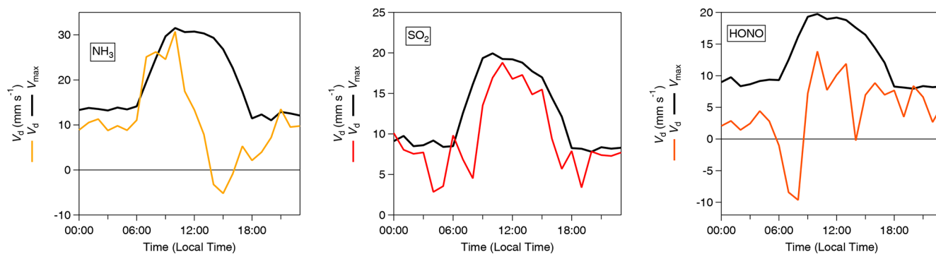
Figure 6. Inorganic trace gas deposition velocities ( V_d ) (post-correction values) with \gamma_F (Chor et al., 2017) and calculated theoretical maximum deposition velocities ( V_{\max} ) for \text{NH}_3 , \text{SO}_2 and HONO.
