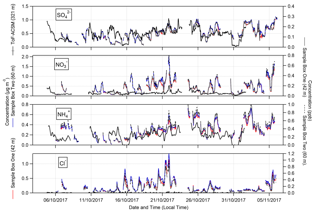
Figure 3. Time series of hourly concentrations (primary left axis, mass concentrations; secondary right axis, molar mixing ratios) of water-soluble aerosol species measured by GRAEGOR at 42 m (red, mass concentration; solid black line, molar mixing ratio) and 60 m (blue, mass concentration; dashed grey line, molar mixing ratio) on the 80 m tower, as well as ToF-ACSM at 321 m (black) at the Amazon tall tower, at the Amazon Tall Tower Observatory site.
