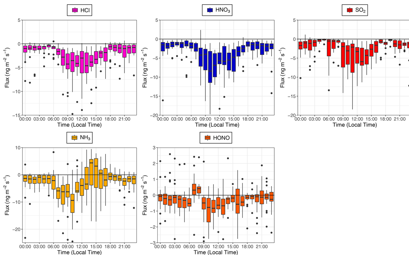
Figure 8. Calculated median diel fluxes of inorganic trace gas species measured during the campaign. From top left (clockwise) – HCl, HNO 3 , SO 2 , HONO and NH 3 . The lower and upper edges of each box correspond to the first and third quartiles, respectively, while the whiskers extend to the largest and smallest values which do not exceed 1.5 times the inter-quartile range from their respective hinge. Black dots outside the plots are values which exceed 1.5 times the inter-quartile range.
