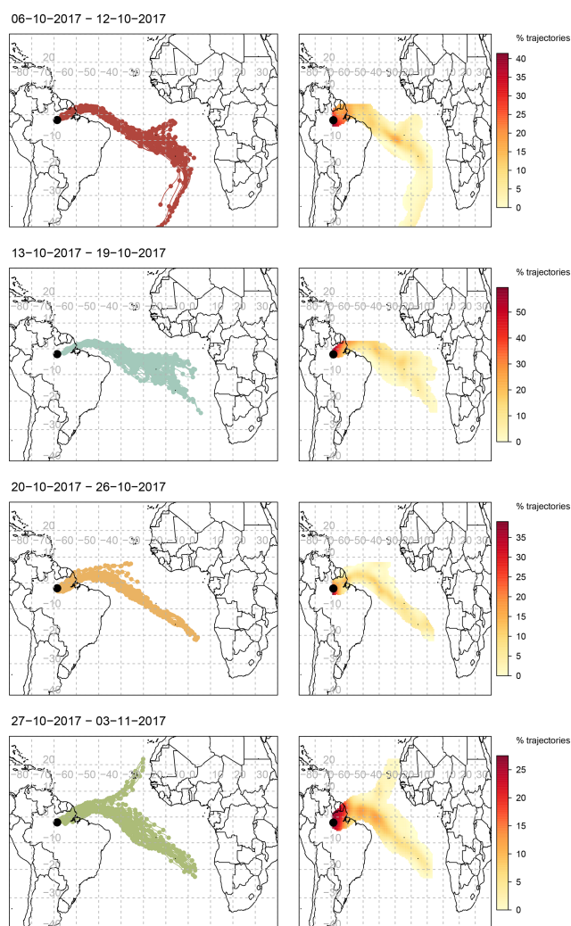
Figure 11. Air-mass back-trajectories arriving at the 80 m walk-up tower on each day every 3 h from 00:00 local time over the period from 6 October to 3 November 2017, grouped by week, and coupled with associated frequency trajectory plots. The duration of each trajectory is 10 d, marks indicate 12 h intervals. Modelled using NOAA HYSPLIT-4 using GDAS1 meteorology.
