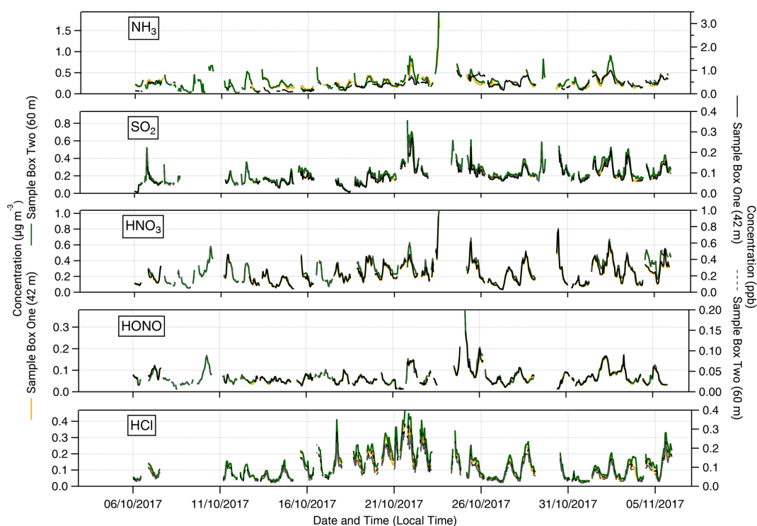
Figure 2. Time series of hourly concentrations (primary left axis, mass concentrations; secondary right axis, molar mixing ratios) of inorganic trace gas species measured by GRAEGOR at 42 m (yellow, mass concentration; solid black line, molar mixing ratio) and 60 m (green, mass concentration; dashed grey line, molar mixing ratio) on the 80 m tower at the Amazon Tall Tower Observatory site.
