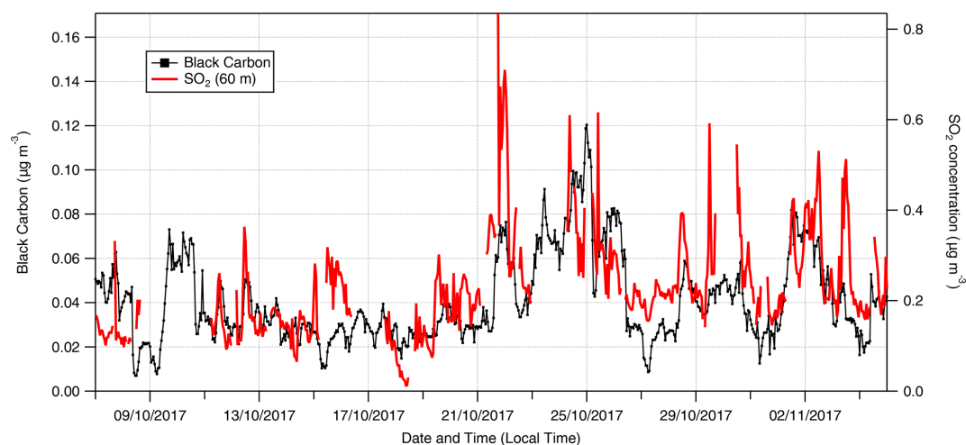
Figure 12. Time series of hourly \text{SO}_2 and \text{BC}_e concentrations, highlighting the close correlation between \text{SO}_2 and \text{BC}_e measurements throughout the campaign.
