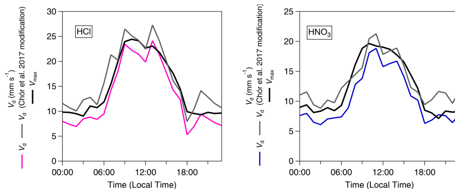
Figure 5. Inorganic trace gas deposition velocities ( V_d ) pre- and post-correction values with \gamma_F (Chor et al., 2017) and calculated theoretical maximum deposition velocities ( V_{\text{max}} ) for \text{HCl} and \text{HNO}_3 .
