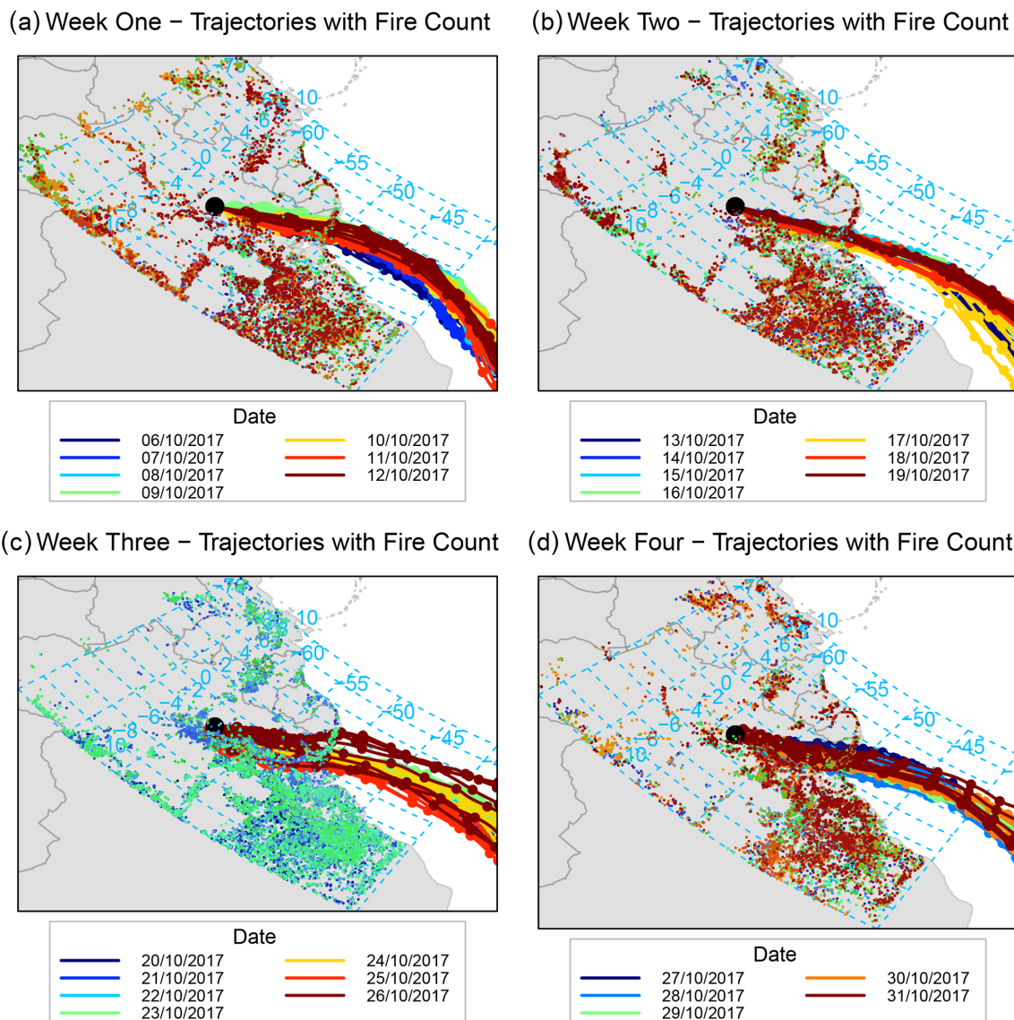
Figure A1. Air-mass back-trajectories arriving at the 80 m walk-up tower on each day every 3 h from 00:00 local time over the period from 6 October 2017 to 31 October 2017, grouped by week, and further subdivided by day, for the regional area surrounding the ATTO site. Fire count data are included as an overlay to each weekly plot, with fire count coloured according to the date on which the fire was recorded by satellite imagery.
