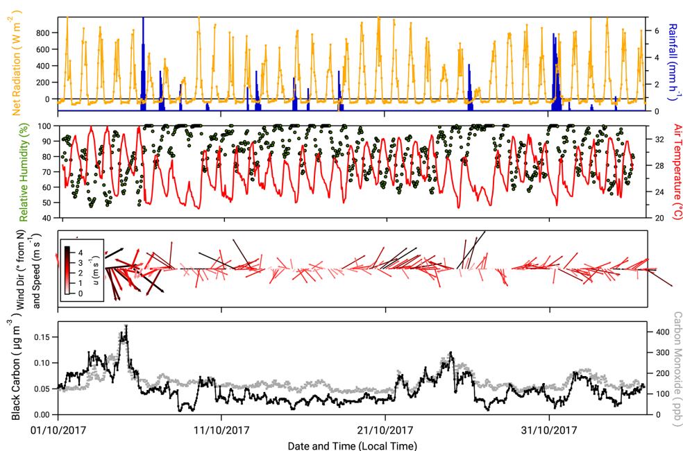
Figure 1. Meteorological and supplementary measurements taken during the campaign. From top, net radiation, hourly rainfall, relative humidity, air temperature, wind speed and wind direction (arrows scaled to wind speed and orientated from 0° N) and concentrations of black carbon and carbon monoxide.
