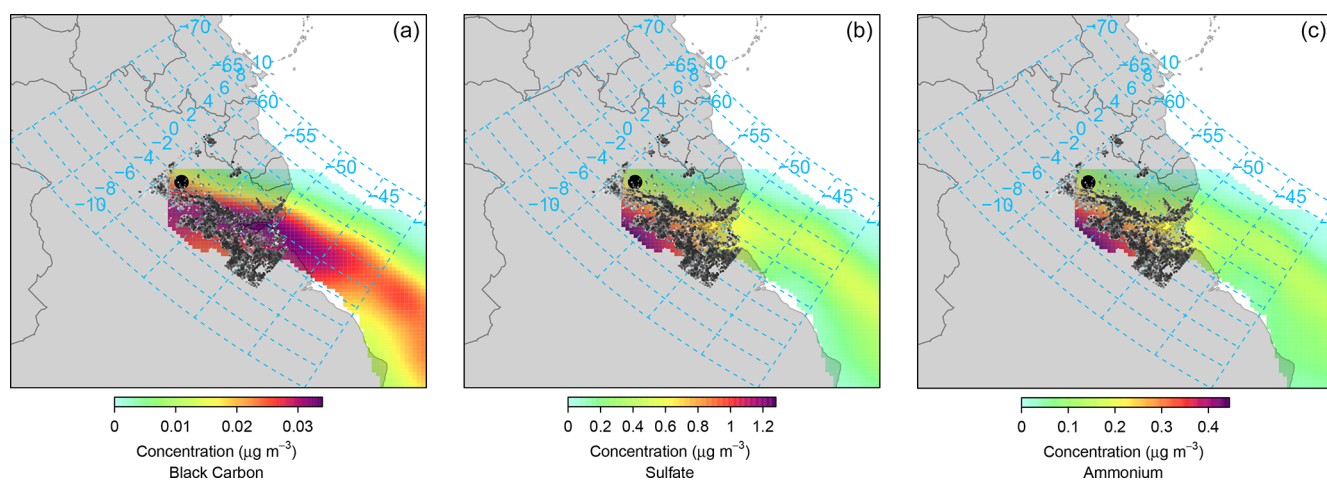
Figure A2. Concentration-weighted trajectory analysis for (from left) \text{BC}_e , \text{SO}_4^{2-} and \text{NH}_4^+ , with fire data overlaid. Fire data are coloured (scale, from light grey to black) by fire intensity, a measure of the fire radiative power of the individual fire.
