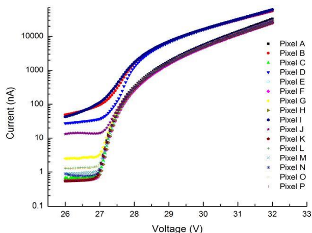
Fig.3 Measured I-V characteristics of all 16 pixels of the ArraySL-4 module.
