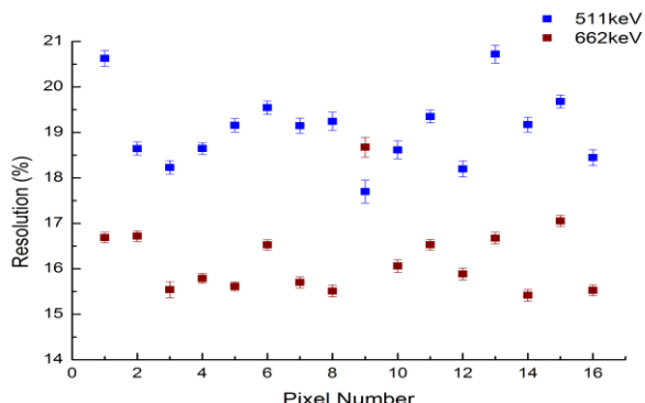
Fig.5 Extracted pixel-to-pixel variations of energy resolutions with gamma-ray energies of 511keV and 662keV.
