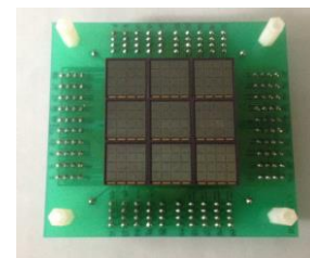
Fig.2 An adapt circuit board made for ArraySM-4p9 module to lead its 144 pixel signals out for individual pixel measurements.
