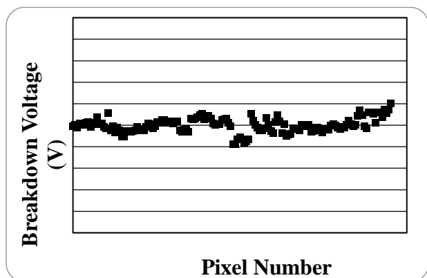
Fig.6 Extracted breakdown voltage pixel-to-pixel variations of ArraySM-4p9 over all the 144 pixels.
