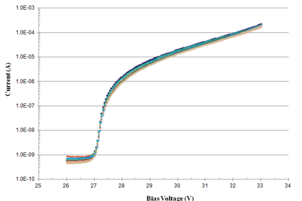
Fig.5 Measured I-V characteristics of 16 pixels from one of the 3x3 units of the ArraySM-4p9 module.
