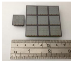
Fig.1 Photo of two SensL's SiPM array modules: ArraySL-4 (4x4 pixels) in left and ArraySM-4p9 (12x12 pixels) in right.
