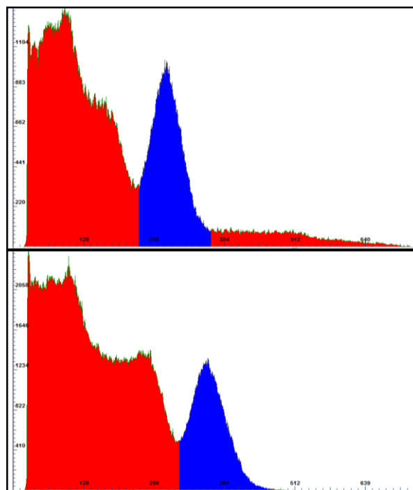
Fig.3 Measured energy spectrum from a typical SiPM pixel with a 1 \times 1 \times 3 \text{mm}^3 LYSO crystal using ^{22}\text{Na} (top) and ^{137}\text{Cs} (bottom) source at bias voltage of 30V.
